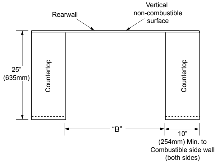
COUNTERTOP CABINET DIMENSIONS (Slide-In, Freestanding Installation)
