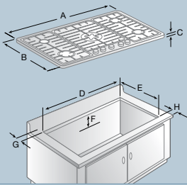
36" Ceramic Gas Cooktop Dimensions
