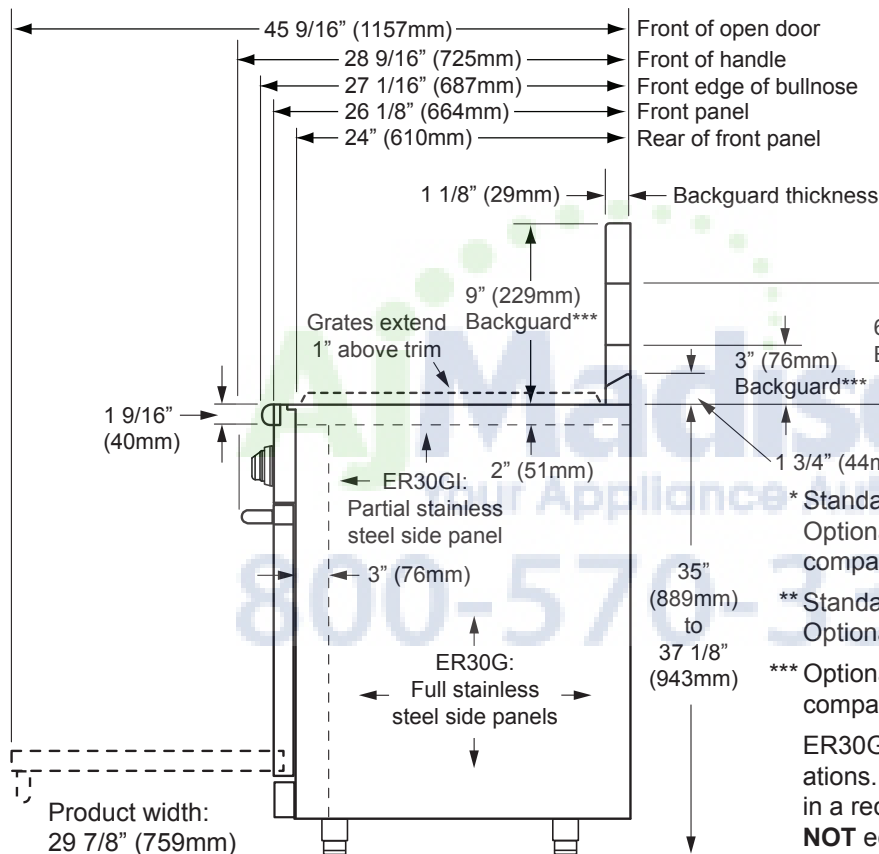
ER30G/ER30GI OVERALL DEPTH DIMENSIONS SIDE VIEW
