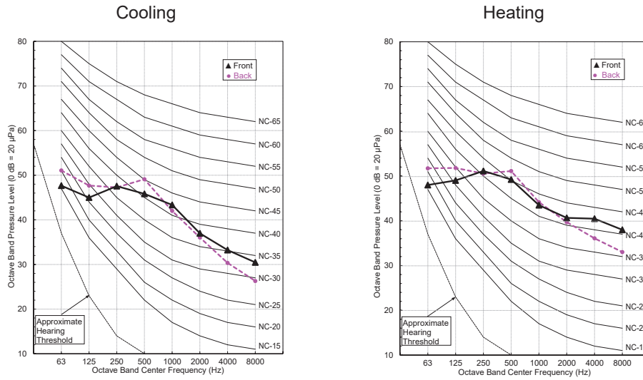
Figure 17: Sound Pressure Levels for Mega 115V LSU120HXV2 Outdoor Units.
