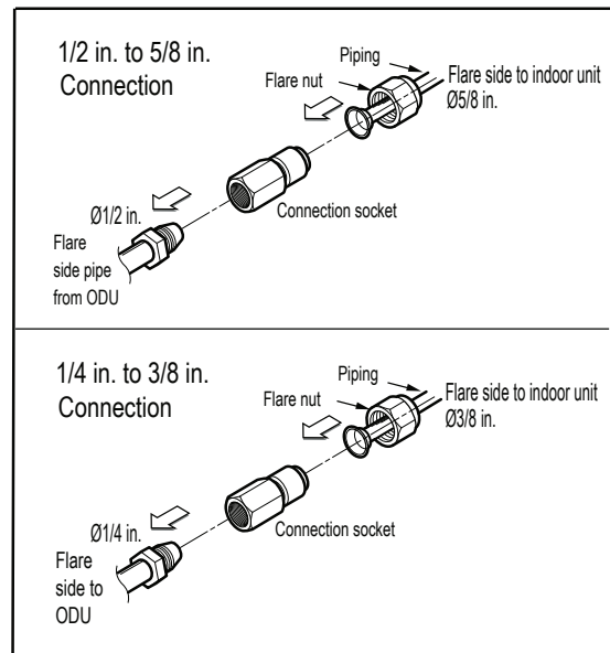
Figure 46: KNUDB181A Refrigerant Pipe Connections.
