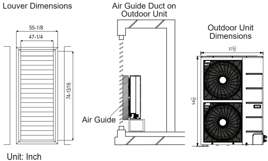
Figure 42: Example of Installing Outdoor Unit Indoors.
