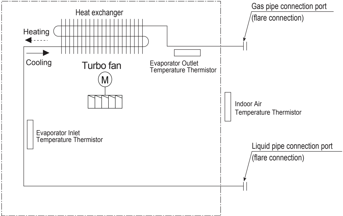
Figure 45: KNUDB091A, KNUDB121A Indoor Unit Refrigerant Flow Diagram.
