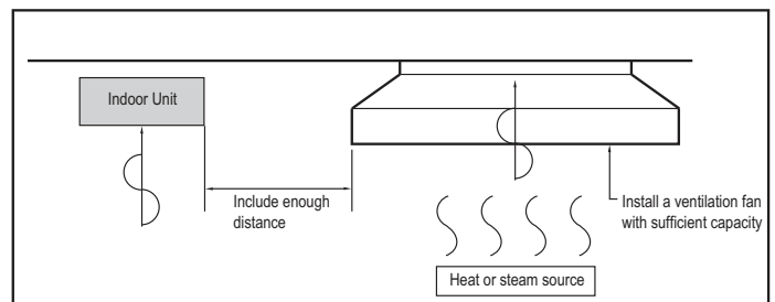
Figure 29: Installing Near a Heat or Steam Source.
