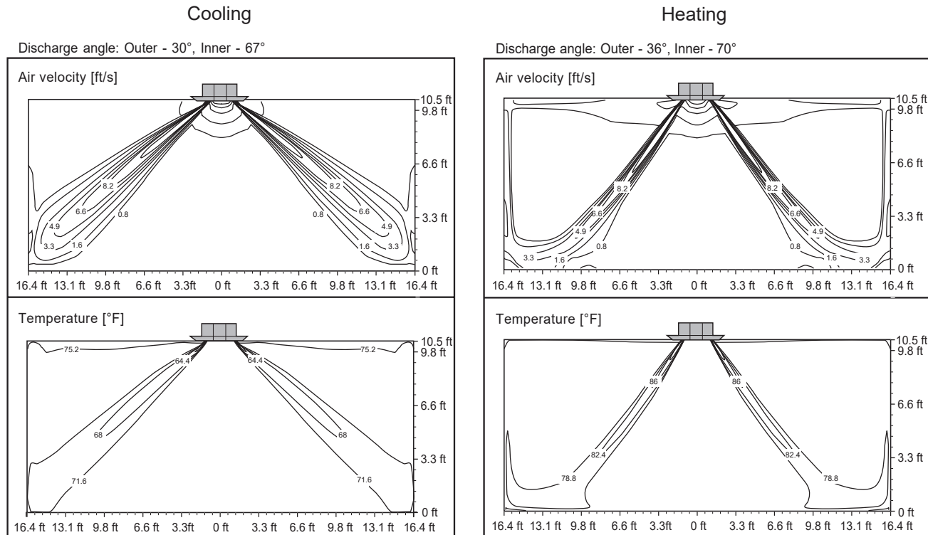
Figure 18: KNCSB301A, KNCSB361A Air Velocity and Temperature Distribution Charts.
