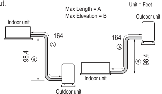
Figure 50: Typical KSUDB181A, KSSCB241A, and KSSCB301A System Layout.
