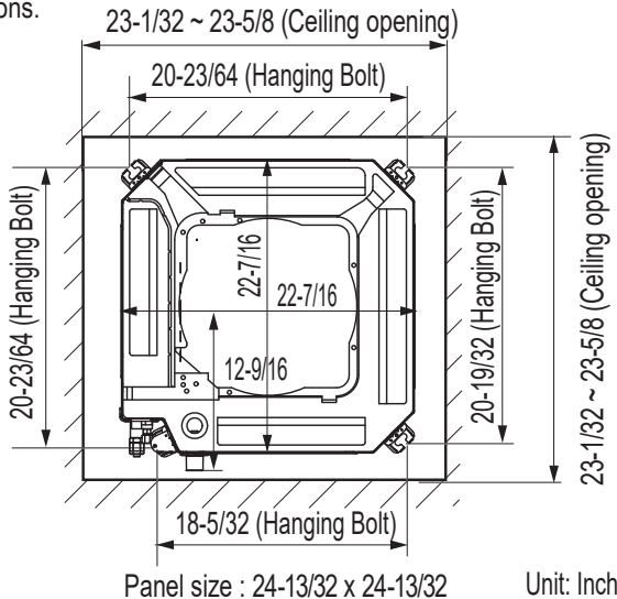
Figure 27: 2 x 2 Cassette Ceiling Opening Dimensions and Bolt Locations.
