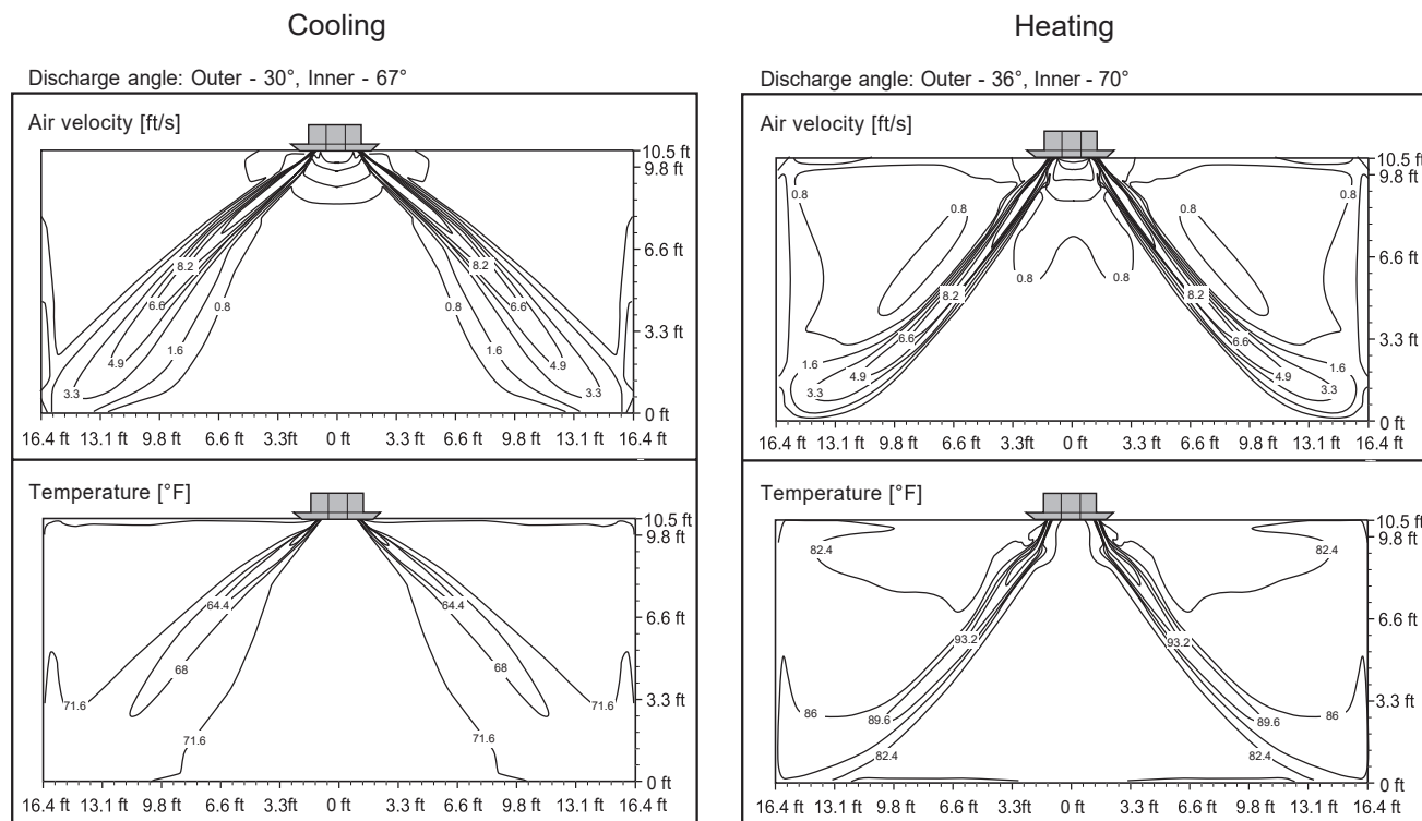
Figure 19: KNCSB421A, KNCSB481A Air Velocity and Temperature Distribution Charts.
