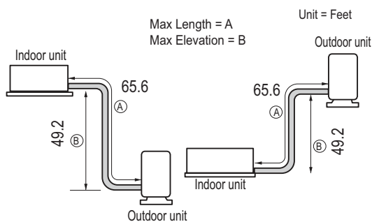
Figure 51: Typical KSSCB361A, KSSCB421A, KSSCB481A System Layout.
