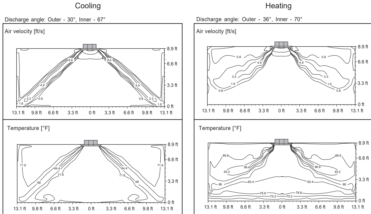
Figure 17: KNSCB241A Air Velocity and Temperature Distribution Charts.
