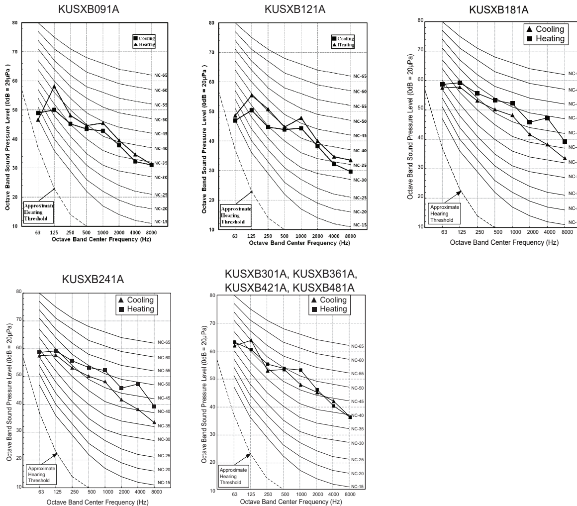
Figure 21: Four-Way Ceiling Cassette Outdoor Unit Sound Pressure Level Diagrams.
