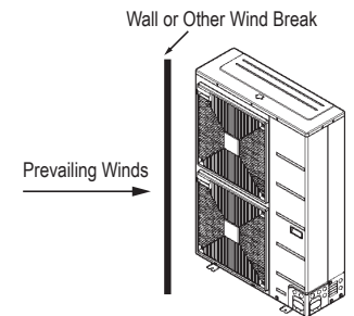
Figure 33: Wind Break.
