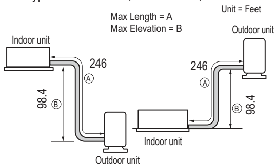
Figure 51: Typical KSSCB361A, KSSCB421A, KSSCB481A System Layout.
