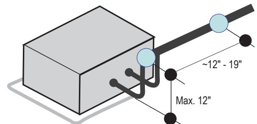
Figure 56: Pipe Support at Indoor Unit.
