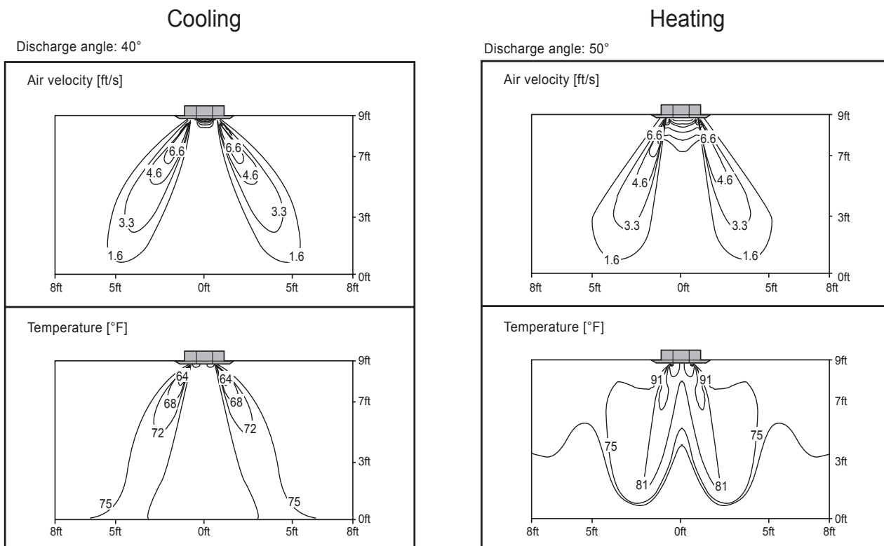
Figure 15: KNUDB121A Air Velocity and Temperature Distribution Charts.
