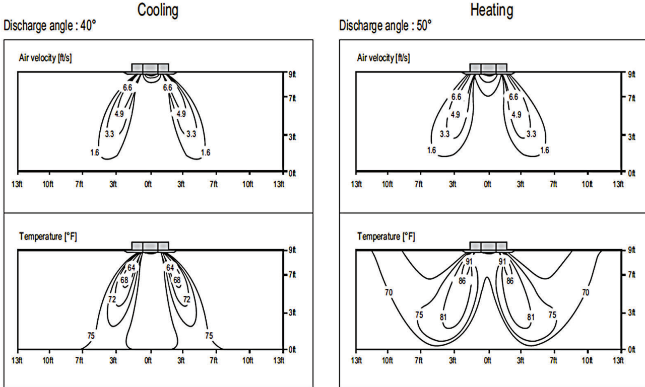
Figure 16: KNUDB181A Air Velocity and Temperature Distribution Charts.
