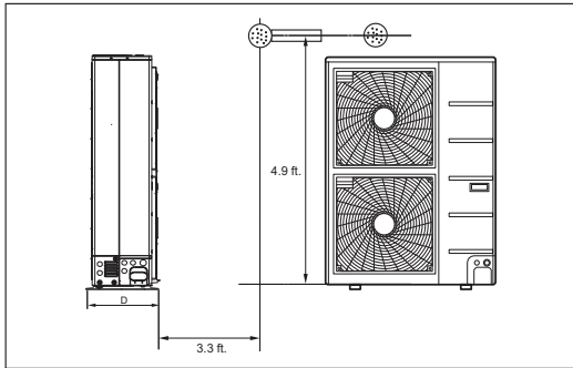
Figure 20: Four-Way Ceiling Cassette Outdoor Unit Sound Pressure Level Measurement Location (For Illustrative Purposes Only; Appearance Depends on Model).
