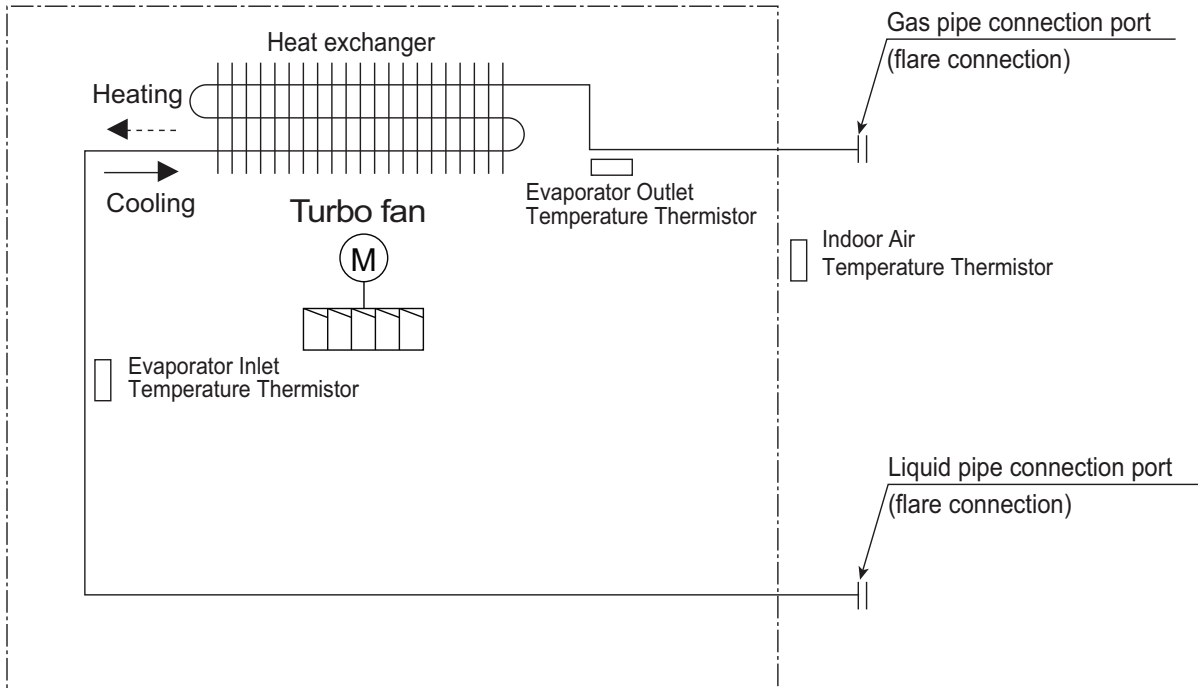
Figure 47: KNUDB181A Indoor Unit Refrigerant Flow Diagram.
