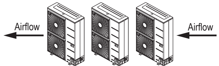
Figure 36: Improper Outdoor Unit Placement.
