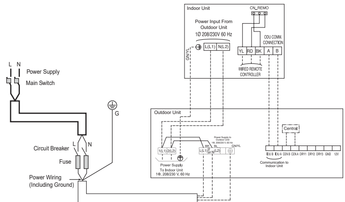
Figure 66: General R32 Single-Zone System Power / Communications System Schematic (Appearances May Vary).
