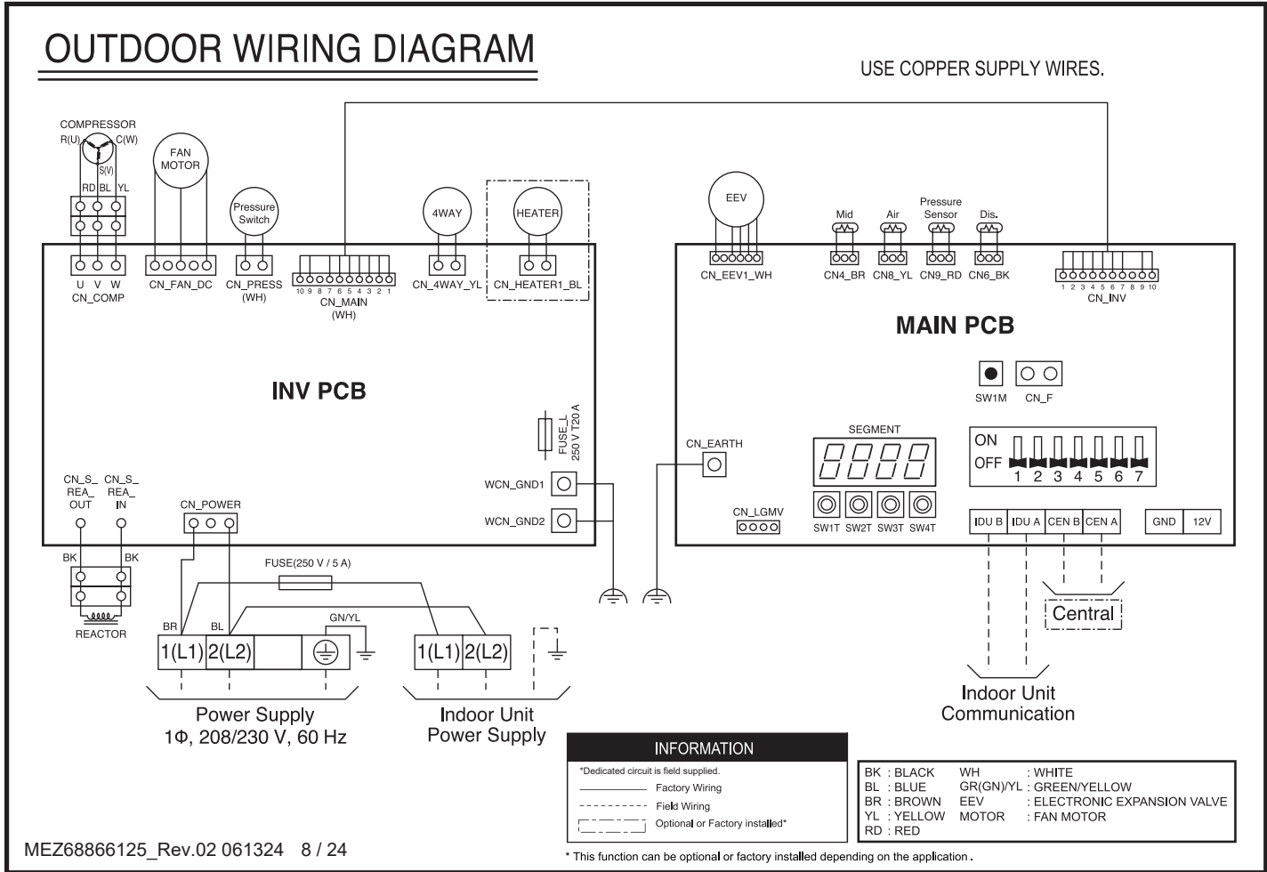
Figure 58: KUSXB091A, KUSXB121A Outdoor Unit Wiring Diagram.
