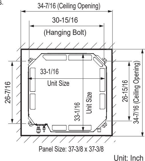
Figure 28: 3 x 3 Cassette Ceiling Opening Dimensions and Bolt Locations.
