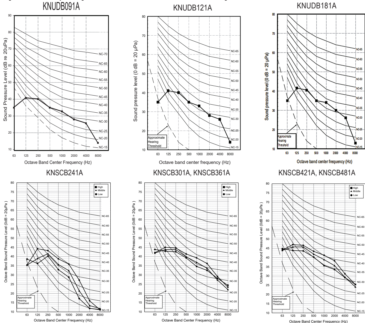
Figure 24: Four-Way Ceiling Cassette Indoor Unit Sound Pressure Level Diagrams.
