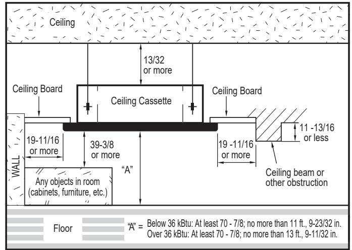
Figure 26: Cassette Indoor Unit Clearance Requirements.
