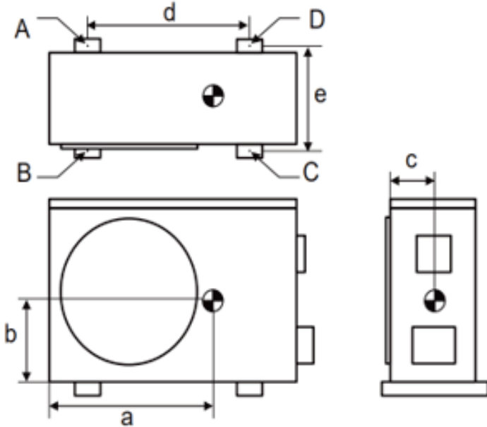
Figure 9: Outdoor Unit Center of Gravity and Corner Weight Diagram.
