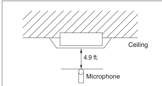
Figure 23: Four-Way Ceiling Cassette Indoor Unit Sound Pressure Level Measurement Location.
