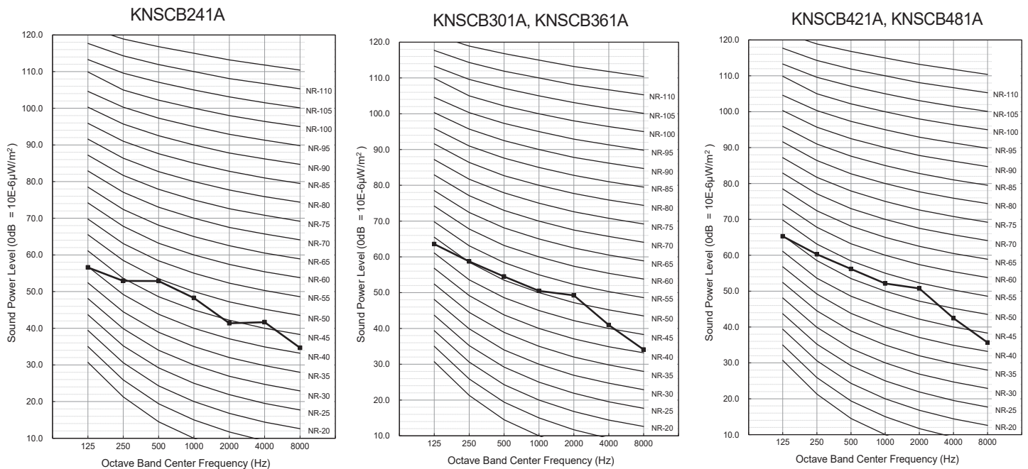
Figure 25: Four-Way Ceiling Cassette Indoor Unit Sound Power Level Diagrams.
