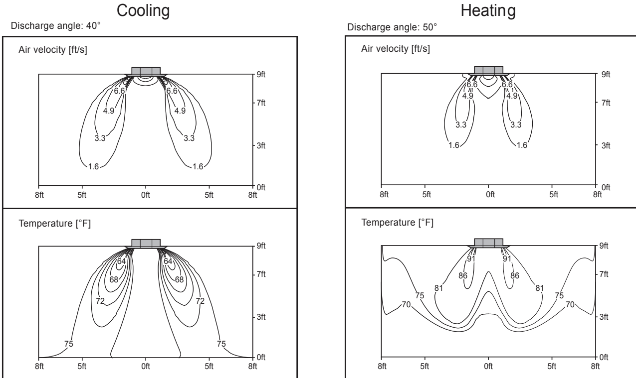
Figure 15: KNUDB121A Air Velocity and Temperature Distribution Charts.
