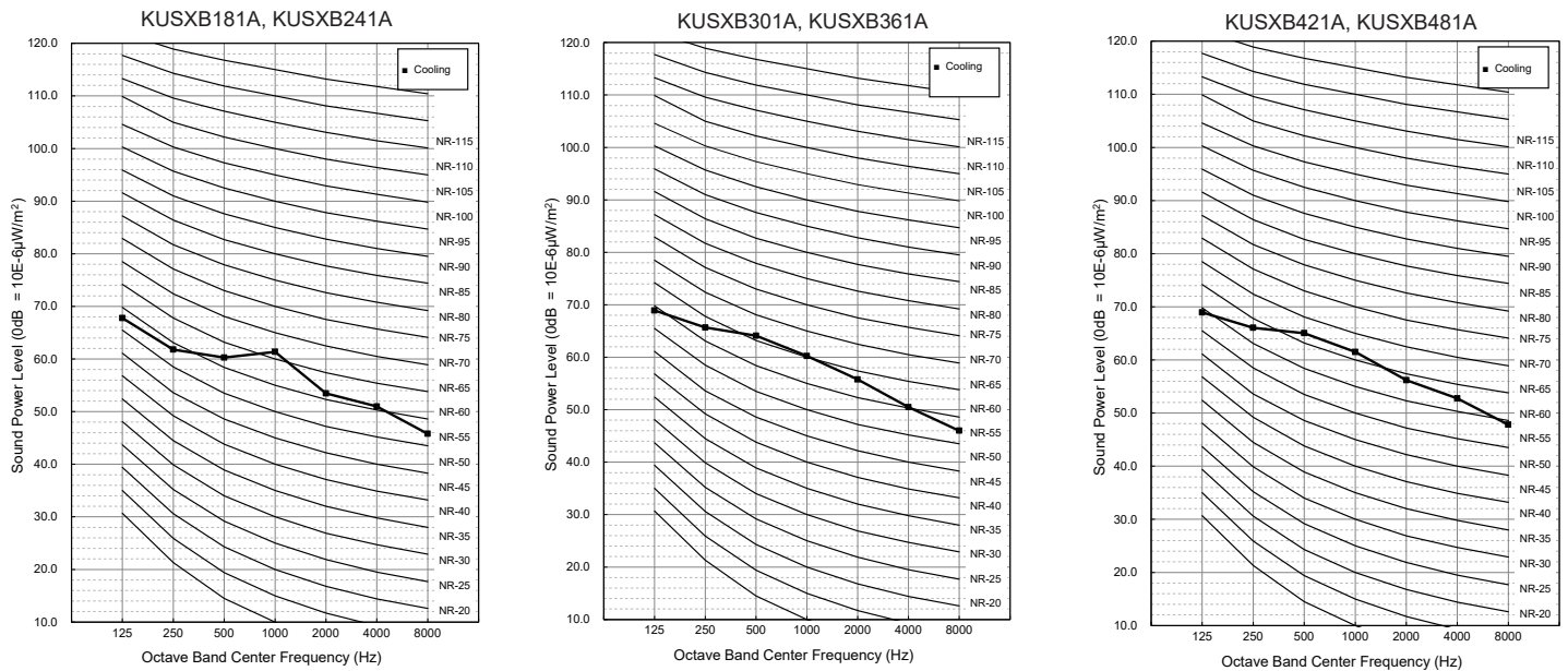
Figure 22: Four-Way Ceiling Cassette Outdoor Unit Sound Power Level Diagrams.
