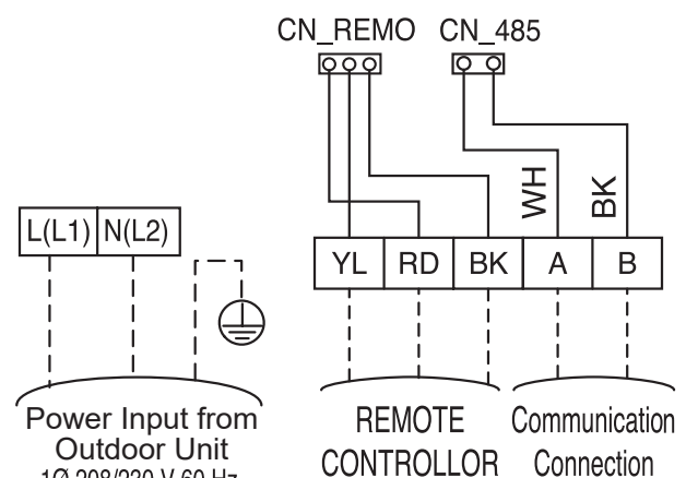
Figure 71: Wired Controller Connection (Example Only).
