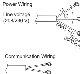
Figure 69: R32 Single-Zone Power / Communication Terminals (Appearances May Vary Slightly).
