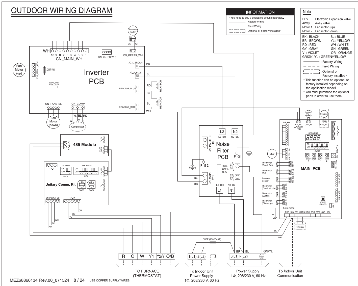
Figure 60: KUSXB421A, KUSXB481A Outdoor Unit Wiring Diagram.
