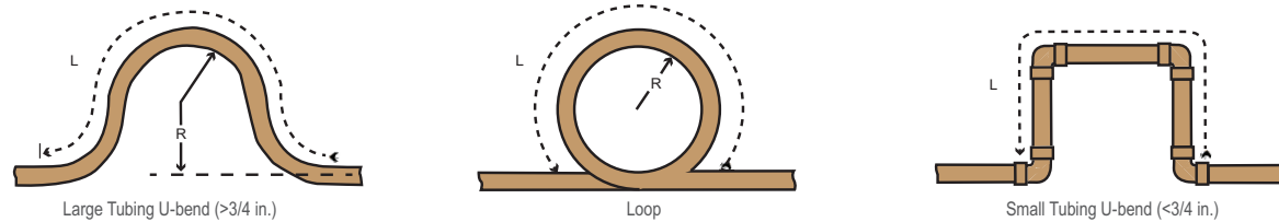
Figure 52: Coiled Expansion Loops and Offsets (Plan View).
