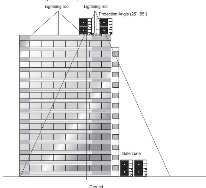
Figure 30: Lightning Protection Diagram (Outdoor Unit Appearances Differ According to Model).
