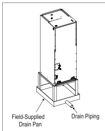
Figure 203: Vertical Installation Drain System.
