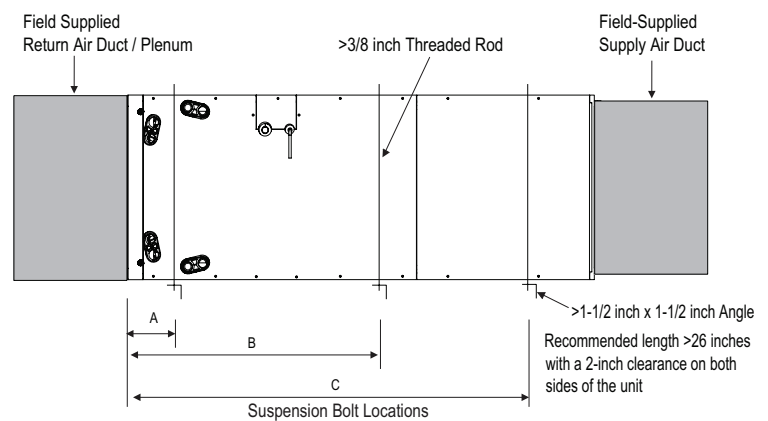
Figure 235: Typical Horizontal Right Installation.
