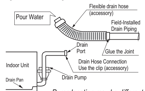
Figure 112: Checking the Drain Pump.
