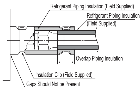
Figure 243: Close Up of Refrigerant Piping Connection Insulation.
