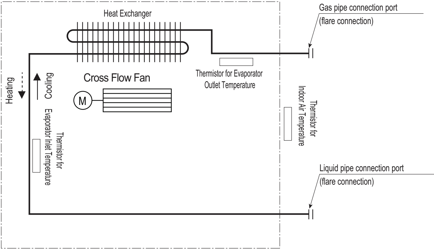
Figure 195: Multi F Vertical-Horizontal Air Handling Indoor Unit Refrigerant Flow Diagram.
