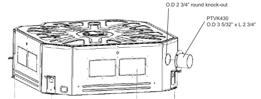
Figure 188:PTVK430 Ventilation Kit.
