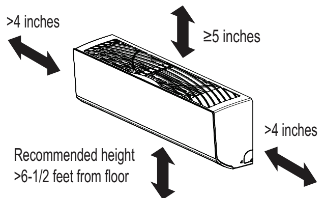
Figure 10: Minimum Clearance Requirements.
