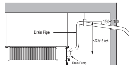
Figure 110: Indoor Unit Using Drain Pump.
