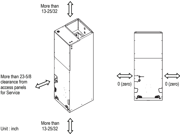
Figure 229:Clearance Requirements.
