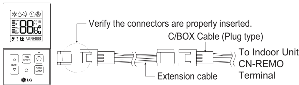
Figure 213:PZCWRC1 LG Wired Remote Extension Cable.
