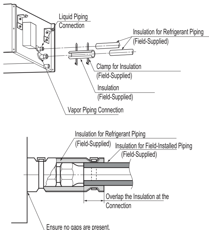
Figure 143: Insulating the Piping.
