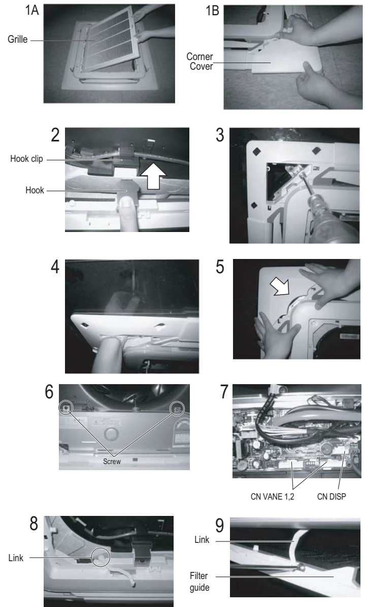
Figure 189:Installing the Decoration Panel.
