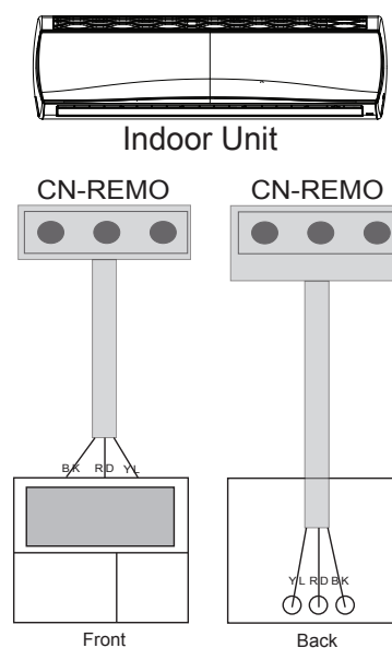
Figure 270: Another Example of Indoor Unit to Zone Controller Connection.
