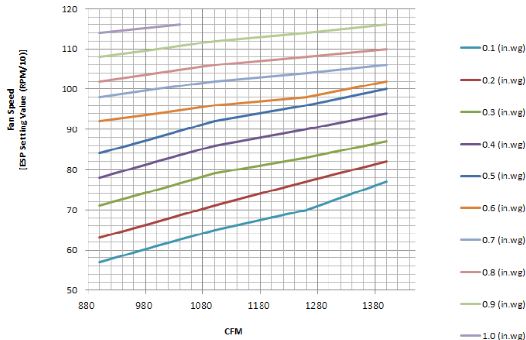
Figure 222: ESP Setting Values – NK Chassis, LVN360HV4.
