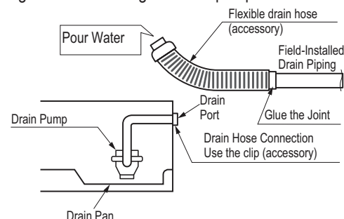
Figure 141: Checking the drain pump.
