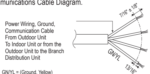
Figure 261: Multi F / Multi F MAX Outdoor and Indoor / Branch Distribution Unit Wiring and Communications Cable Diagram.
