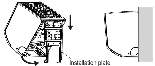
Figure 13: Locking the Indoor Unit onto the Installation Plate.
