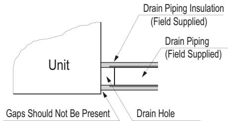
Figure 205: Close up of Drain Piping Connection.
