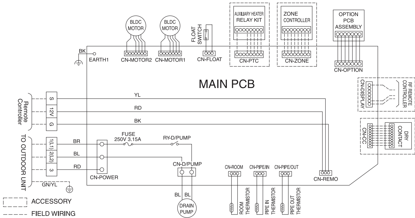
Figure 101:Multi F Ceiling-Concealed Duct (Low Static) LDN097HV4, LDN127HV4, and LMDN186HV Indoor Units Wiring Diagram.
