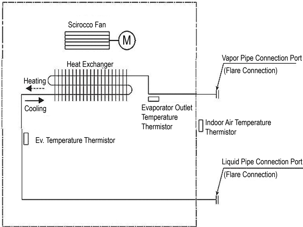
Figure 227: Four-way Vertical-Horizontal Air Handling Indoor Unit Refrigerant Flow Diagram.
