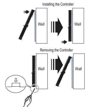
Figure 218: Installing / Removing the Controller.
