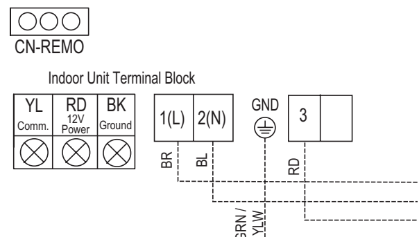
Figure 119:Wired Controller Connections on the Indoor Unit Terminal Block.
