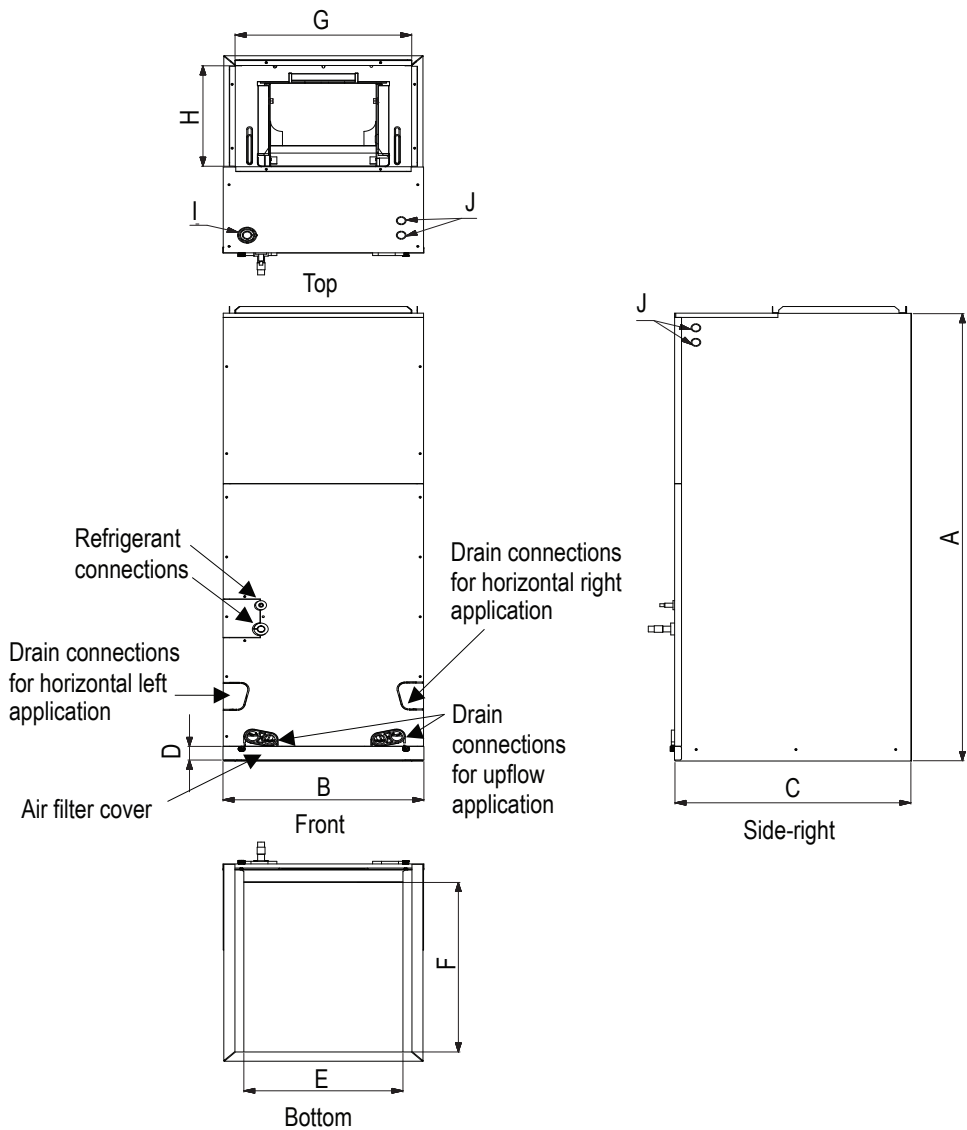
Figure 220: Four-way Vertical Air Handling Unit Dimensions.
