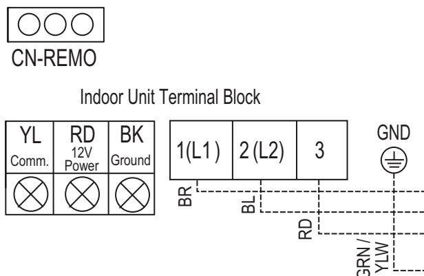
Figure 248:Wired Controller Connection on the Indoor Unit Terminal Block.
