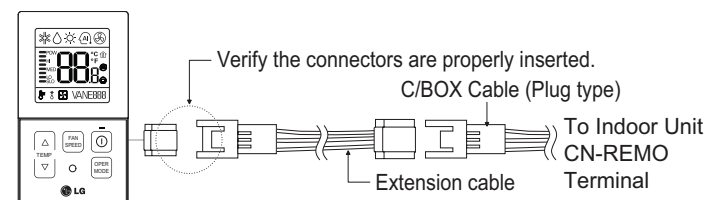
Figure 149: Wired Controller Connections on the Indoor Unit Terminal Block.
