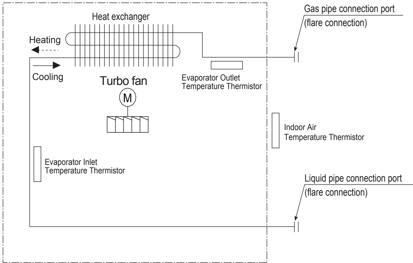
Figure 167: Multi F Four-Way Ceiling-Cassette Indoor Unit Refrigerant Flow Diagram.
