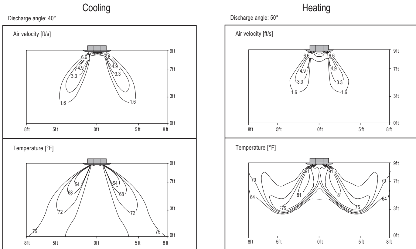
Figure 164:LCN097HV4 Air Velocity and Temperature Distribution Charts.
