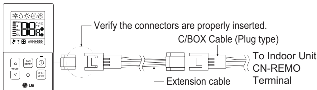
Figure 247:PZCWRC1 LG Wired Remote Extension Cable.
