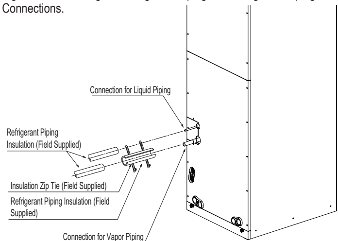
Figure 210: Insulating the Refrigerant Piping and Refrigerant Piping Connections.
