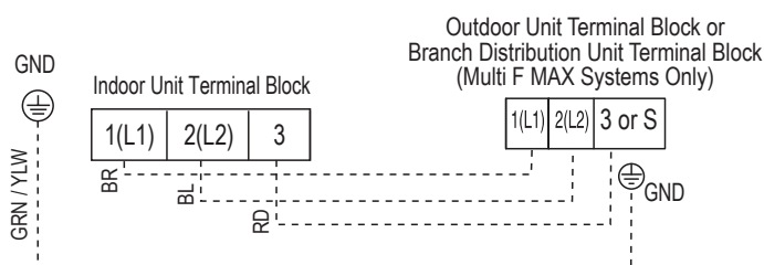
Figure 180: Simplified View of Indoor Unit to Outdoor Unit / Branch Distribution Unit Terminal Connections.
