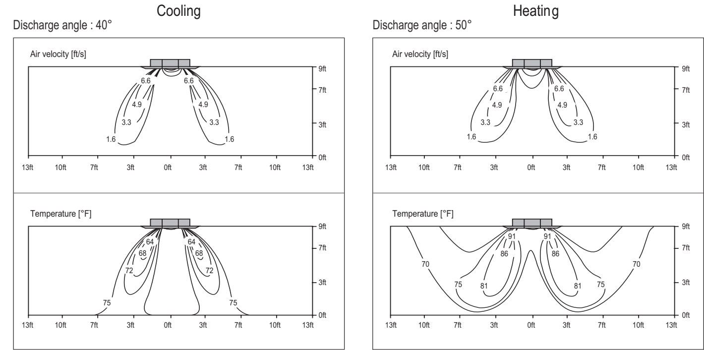
Figure 166:LMCN185HV Air Velocity and Temperature Distribution Charts.
