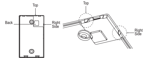
Figure 218: Installing / Removing the Controller.
