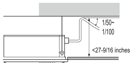
Figure 176: Indoor Unit Drain Piping.
