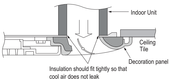
Figure 190:Ensure that no gaps are present between the indoor unit frame and the decoration panel.
