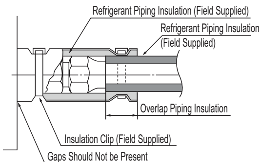
Figure 209: Close Up of Refrigerant Piping Connection Insulation.
