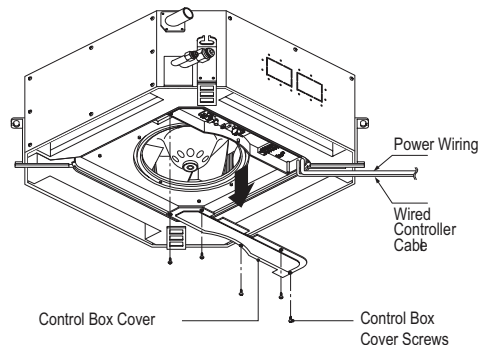
Figure 179: Power Wiring and Communications Cable Connection Access.
