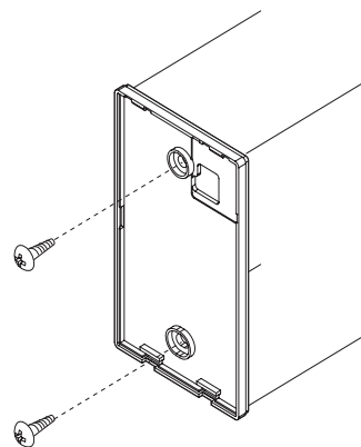
Figure 152: Attaching the Wall Plate.
