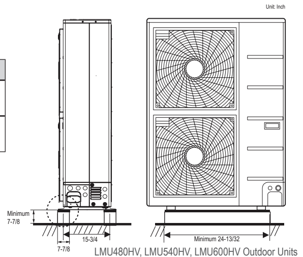
Figure 255: Bolting the Outdoor Unit to the Platform.
