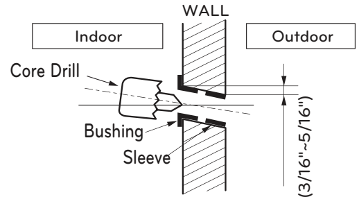
Figure 19: Drilling Piping Hole
