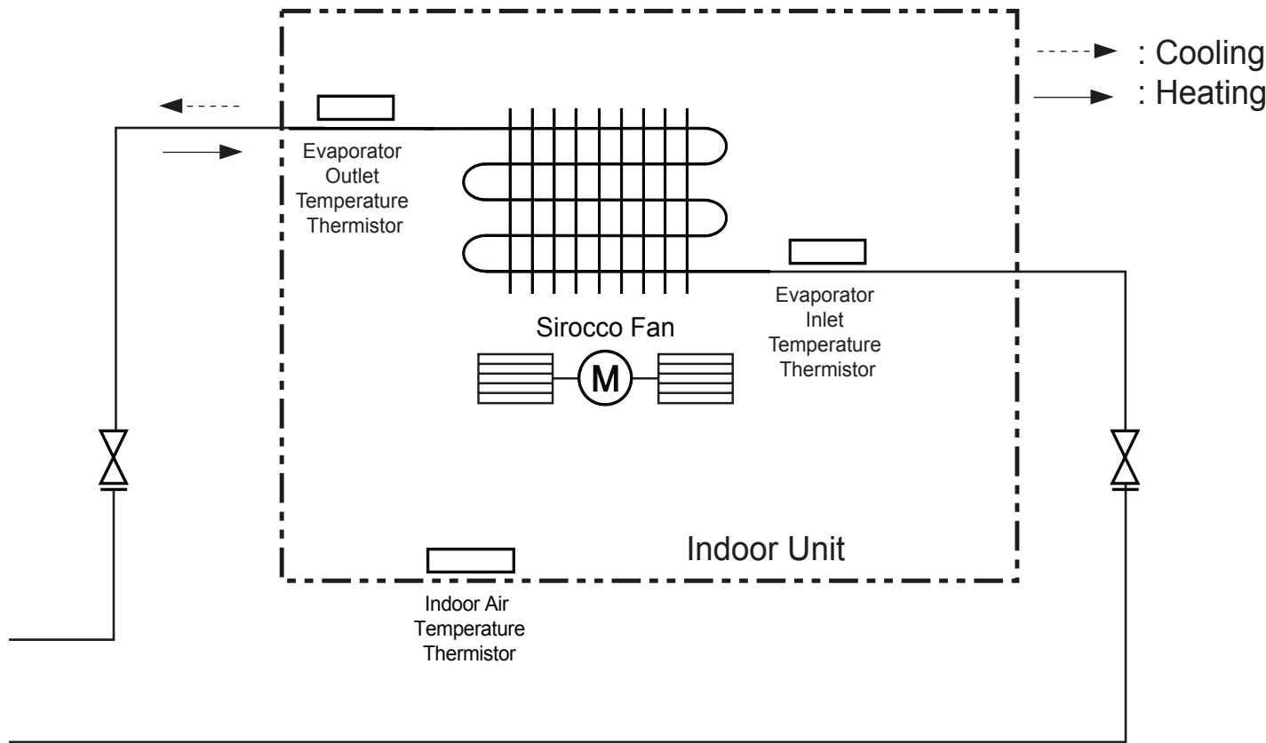
Figure 99: LDN097HV4 Refrigerant Flow Diagram.
