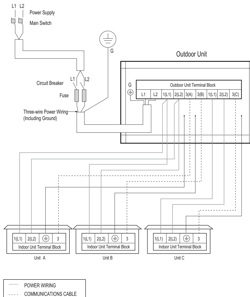
Figure 265: Multi F LMU24CHV System Power Wiring and Communications Cable.
