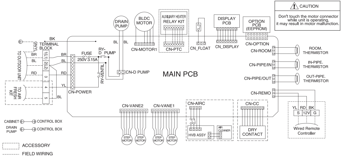
Figure 168: Multi F Four-Way Ceiling-Cassette Indoor Unit Wiring Diagram.
