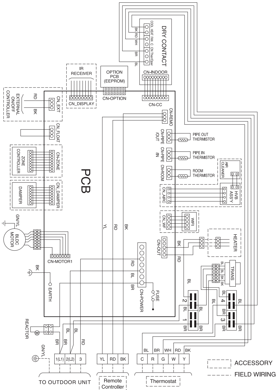
Figure 228: Four-way Vertical-Horizontal Air-Handling Indoor Unit Wiring Diagram.
