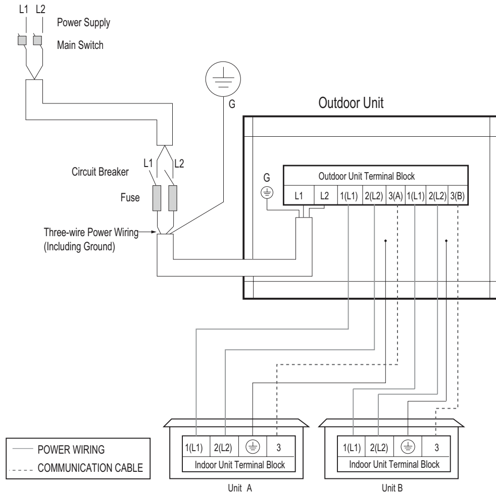
Figure 264: Multi F LMU18CHV System Power Wiring and Communications Cable.
