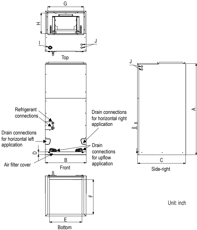
Figure 231:Location of Access Holes and Piping Connections.
