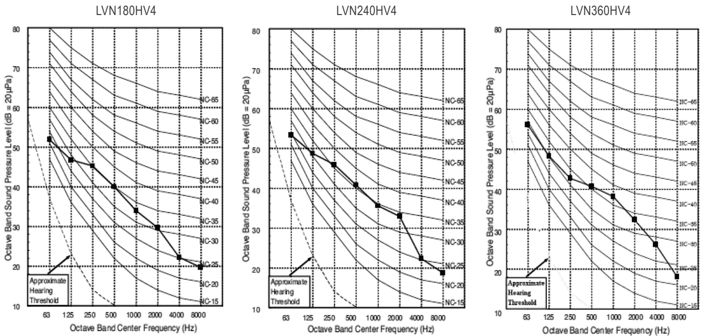
Figure 225: Sound Pressure Level Diagrams.
