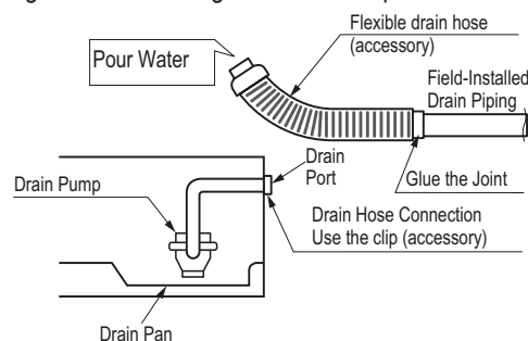
Figure 177: Checking the Drain Pump.
