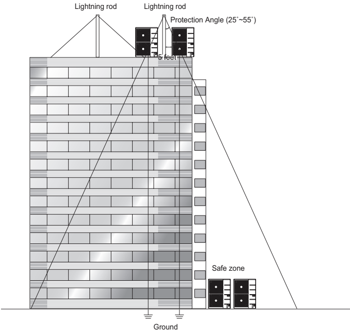
Figure 257: Lightening Protection Diagram.
