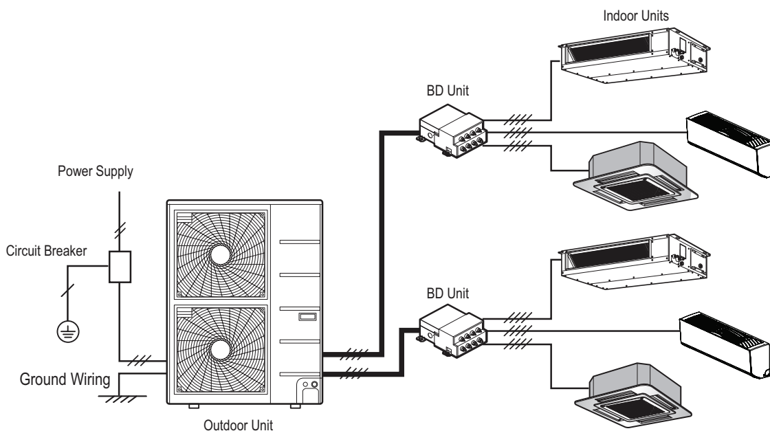
Figure 263: Multi F MAX System General Power / Communications System Schematic.
