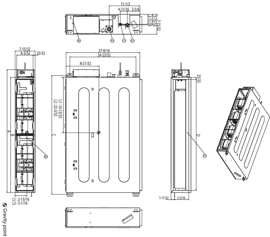
Figure 96:LDN097HV4, LDN127HV4, and LMDN186HV Dimensions.
