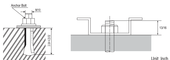
Figure 256: Close up of Bolt Attachment.
