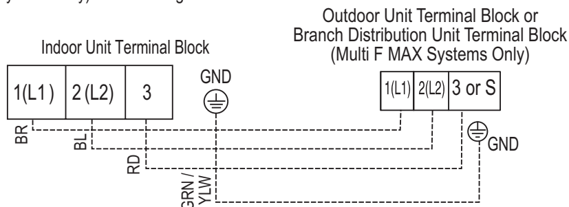
Figure 246: Indoor Unit to Outdoor Unit / Branch Distribution Unit (Multi F MAX systems only) Power Wiring / Communications Cable Connections.
