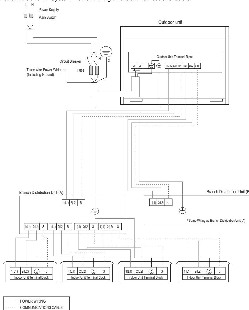
Figure 267: Multi F MAX LMU480HV and LMU540HV System Power Wiring and Communications Cable.
