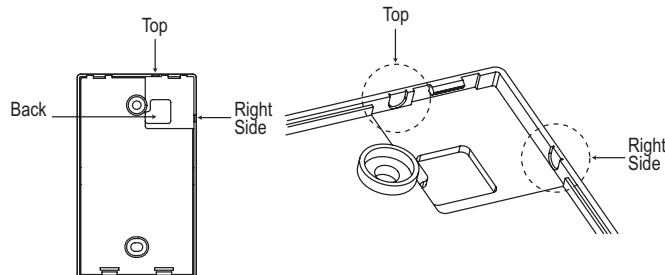
Figure 186: Attaching the Wall Plate.
