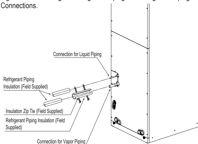
Figure 244: Insulating the Refrigerant Piping and Refrigerant Piping Connections.
