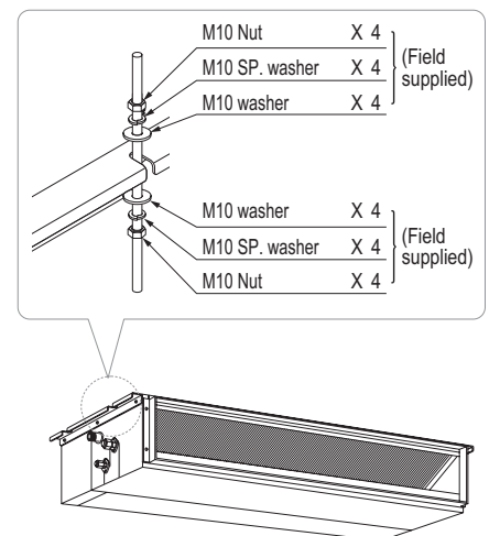
Figure 108: Hanging the Indoor Unit.
