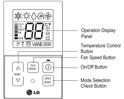
Figure 117:AKB72955816 1 Wired Controller.
