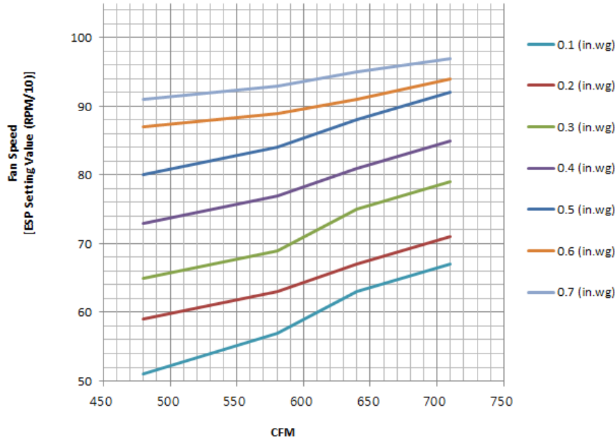
Figure 221: ESP Setting Values – NJ Chassis, LVN180HV4, LVN240HV4
