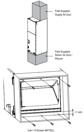
Figure 232: Vertical Installation / Attaching the Bottom Duct.
