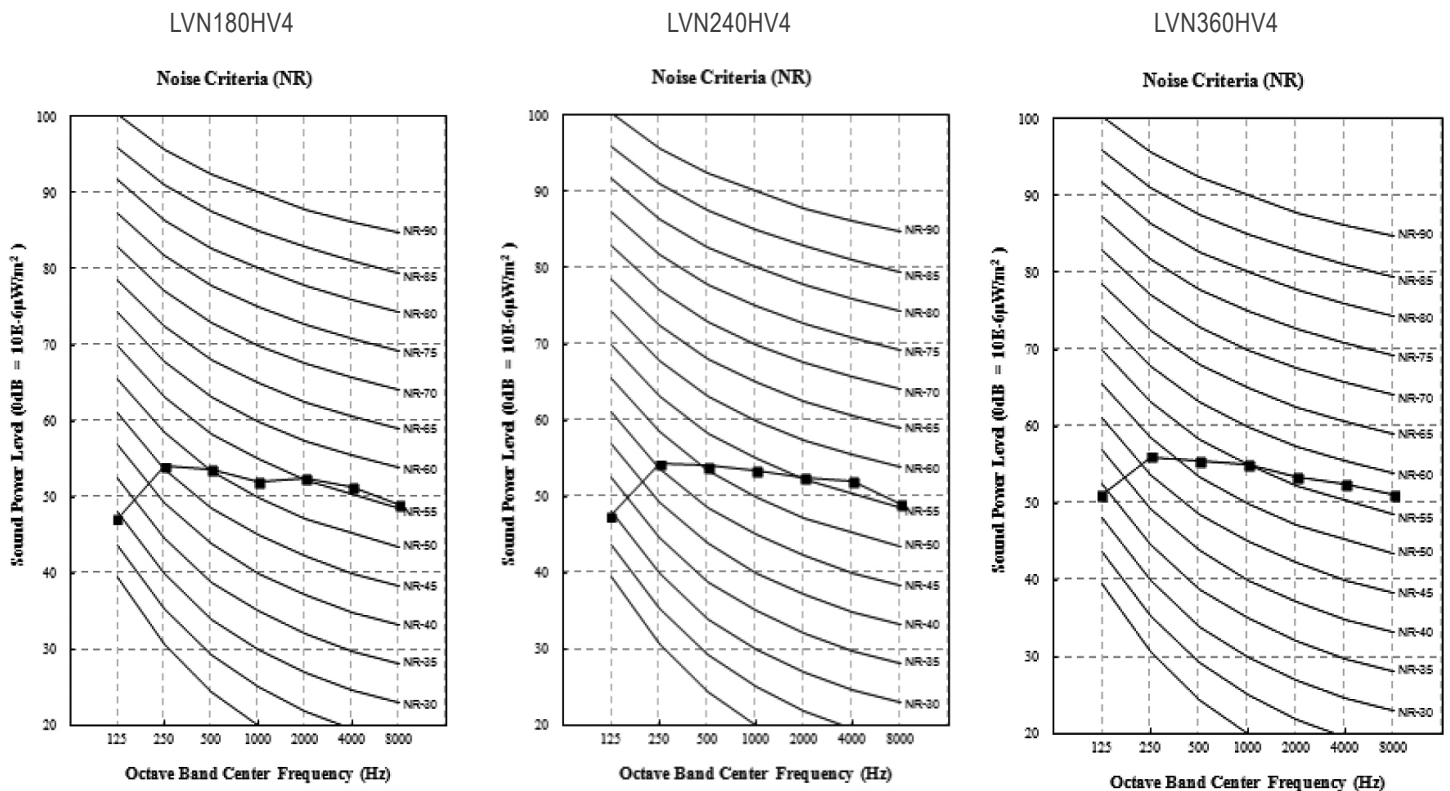
Figure 226: Sound Power Level Diagrams.
