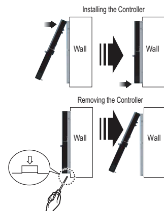
Figure 187: Installing / Removing the Controller.
