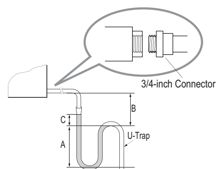
Figure 240: Installing the U-Trap.
