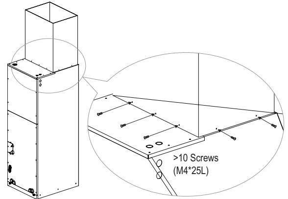
Figure 236: Securing the Ducts to the Unit.
