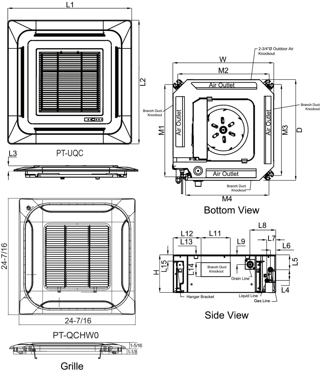
Figure 158:LMCN077HV, LCN097HV4, and LCN127HV4 Dimensions.
