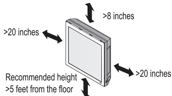
Figure 38: Minimum Clearance Requirements.
