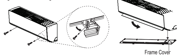
Figure 15: Removing the Frame Cover.
