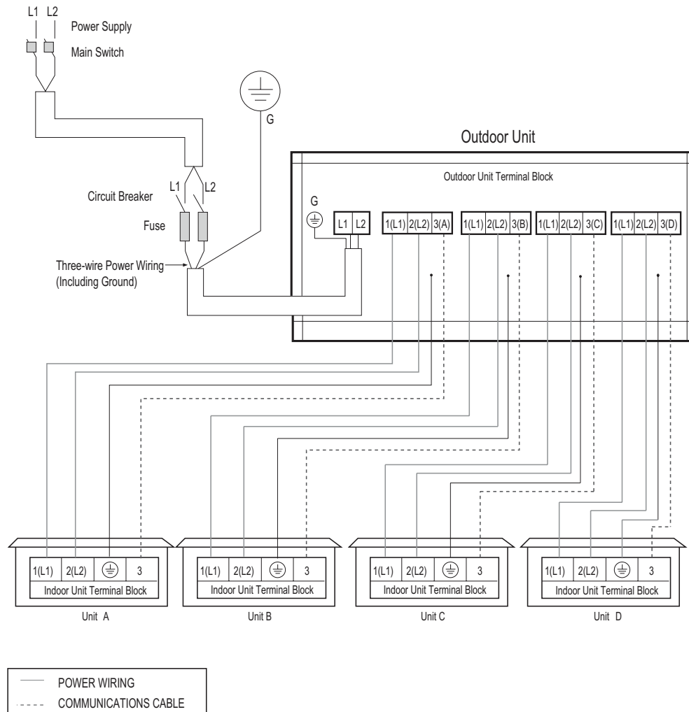
Figure 266: Multi F LMU30CHV and LMU36CHV System Power Wiring and Communications Cable.
