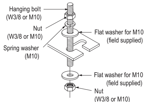
Figure 175: Hanging the Indoor Unit.
