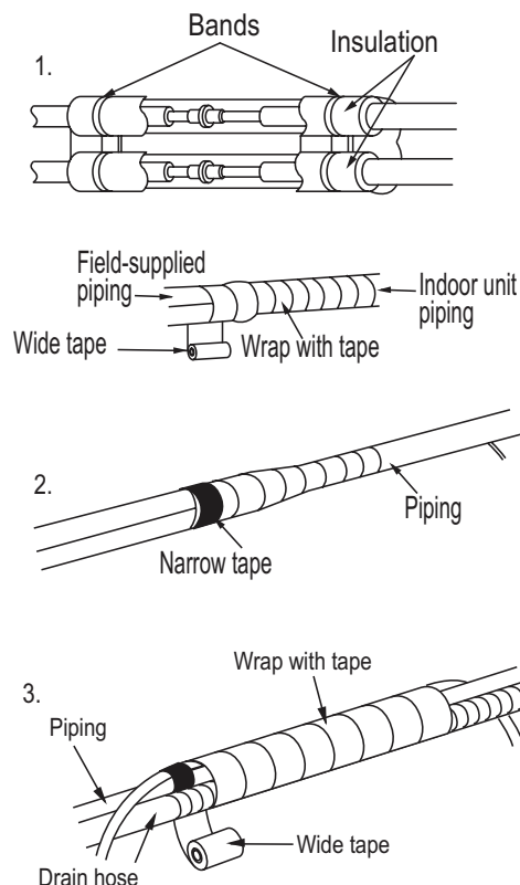
Figure 48: Insulating the Piping.
