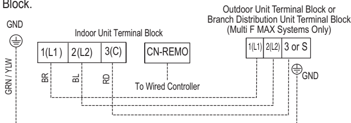
Figure 183:Wired Controller Connection on the Indoor Unit Terminal Block.
