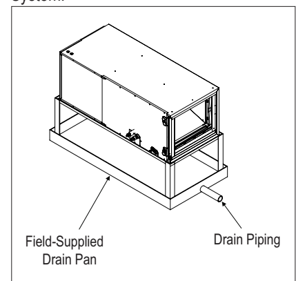
Figure 204: Horizontal Installation Drain System.
