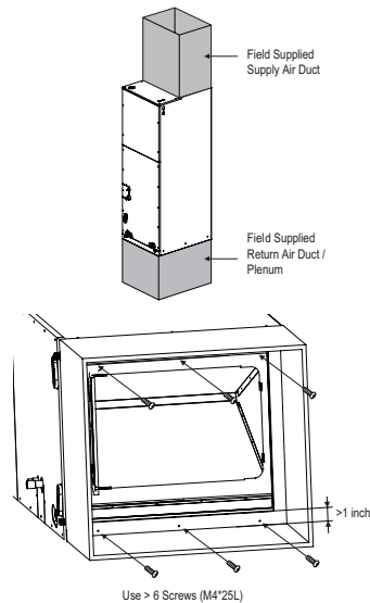
Figure 200:Vertical Installation / Attaching the Bottom Duct.
