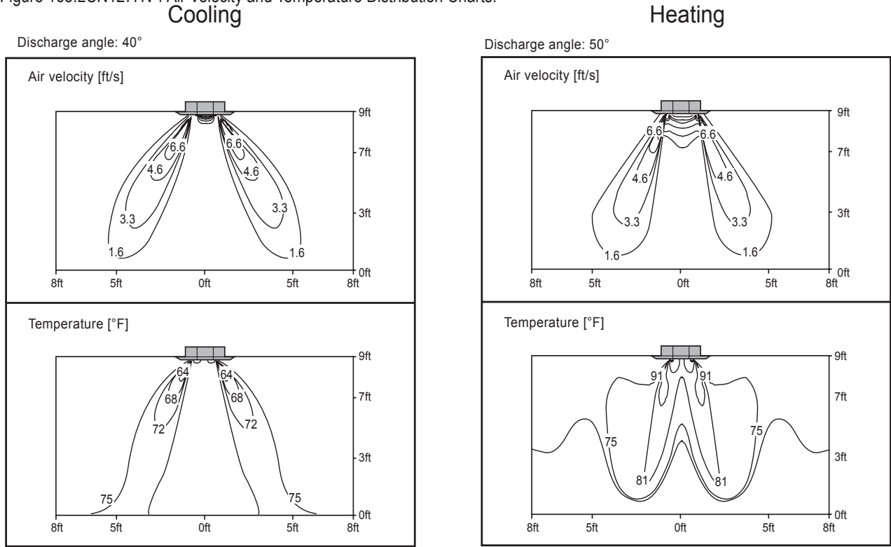
Figure 166:LMCN185HV Air Velocity and Temperature Distribution Charts.
