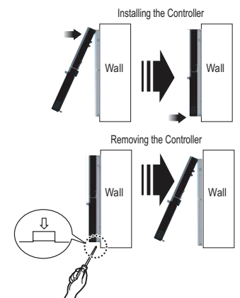
Figure 122: Installing / Removing the Controller.
