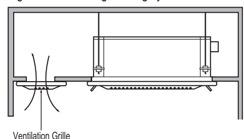
Figure 170: Installing in a Highly Humid Location.
