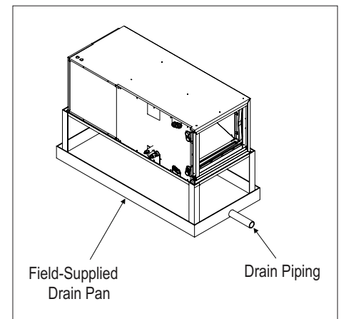
Figure 238: Typical Horizontal Left/Right Installation Drain System.
