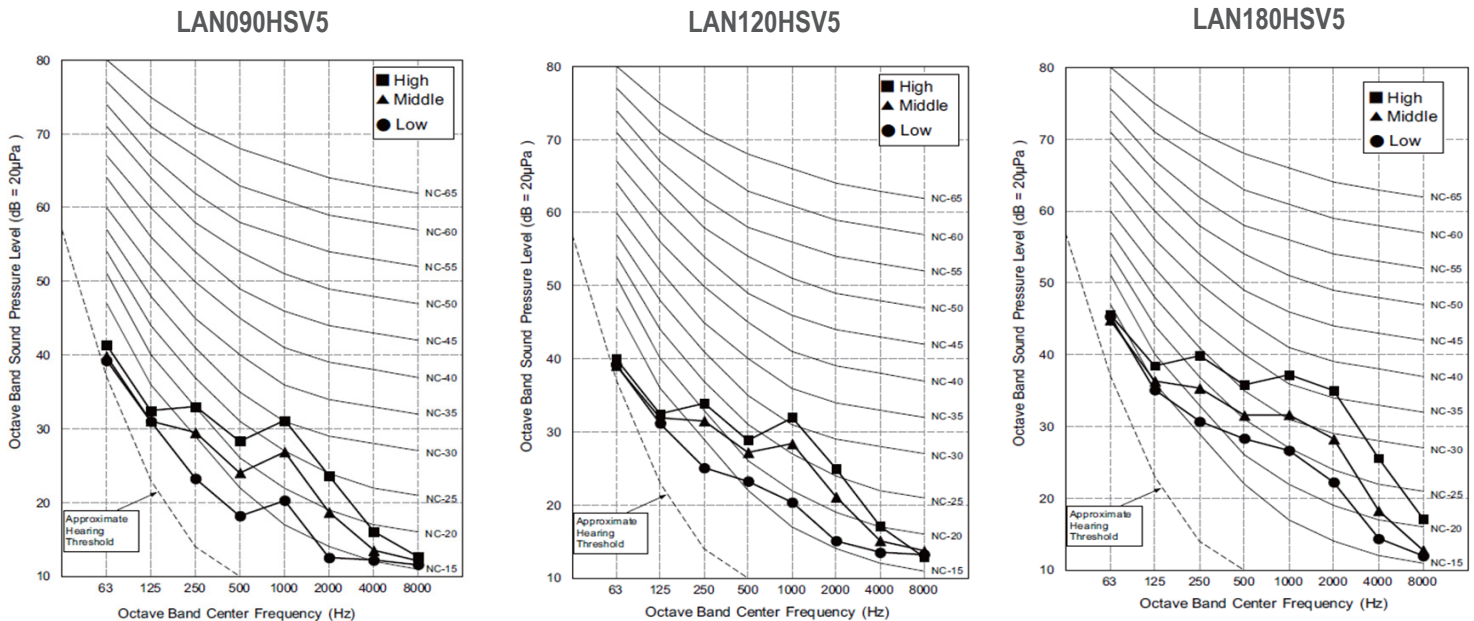
Figure 5: Sound Pressure Level Diagrams.
