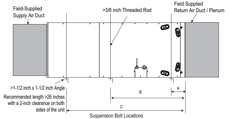
Figure 234: Typical Horizontal Left Installation.
