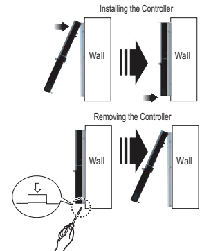
Figure 252: Installing / Removing the Controller.
