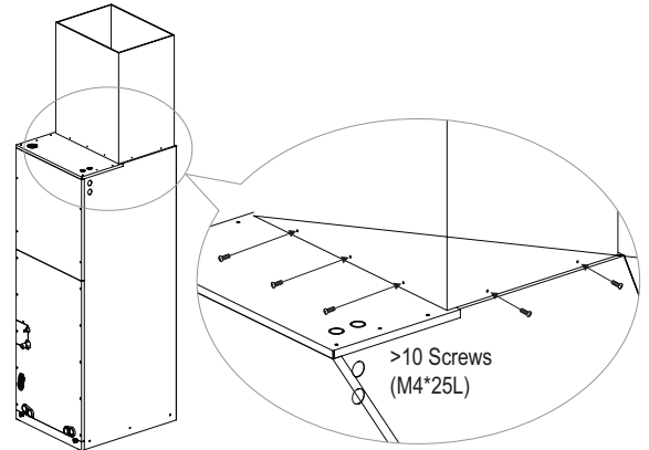
Figure 202: Securing the Ducts to the Unit.
