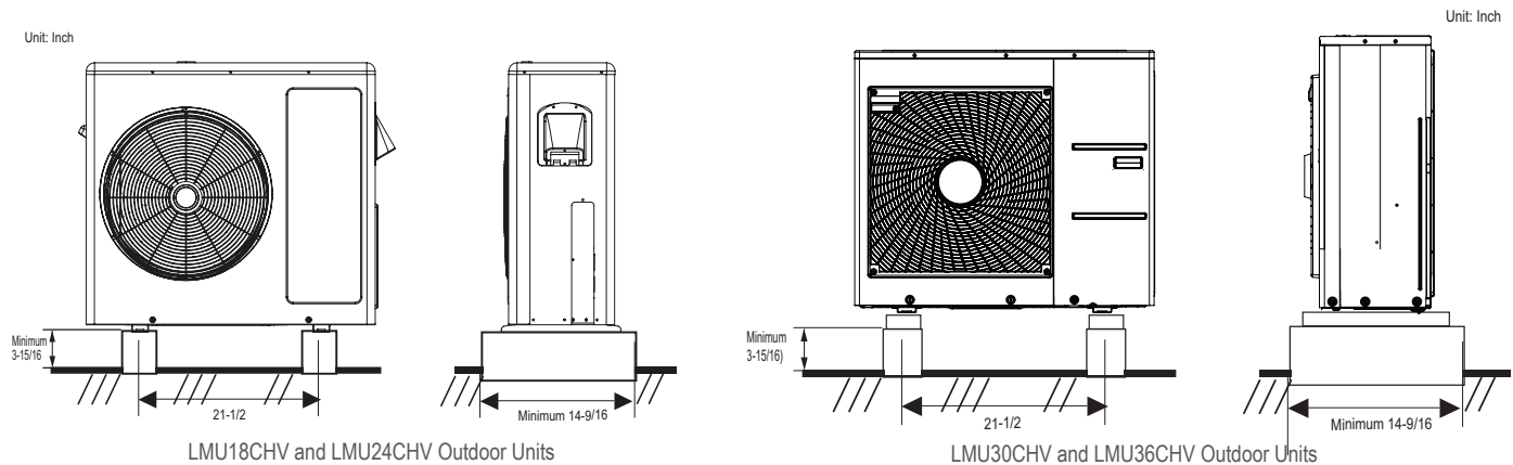
Figure 254: Outdoor Unit Foundation Requirements.
