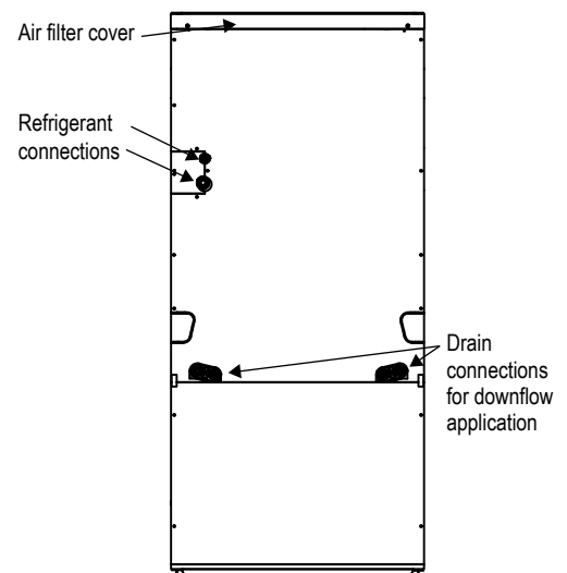
Figure 233: Chassis after Downflow Field Conversion.
