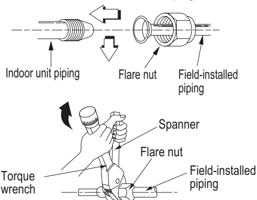
Figure 46: Indoor Unit to Field-Installed Piping Connection.
