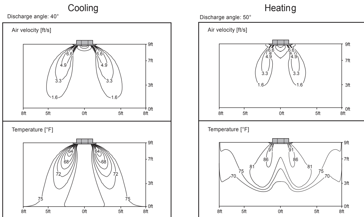
Figure 164:LCN097HV4 Air Velocity and Temperature Distribution Charts.
