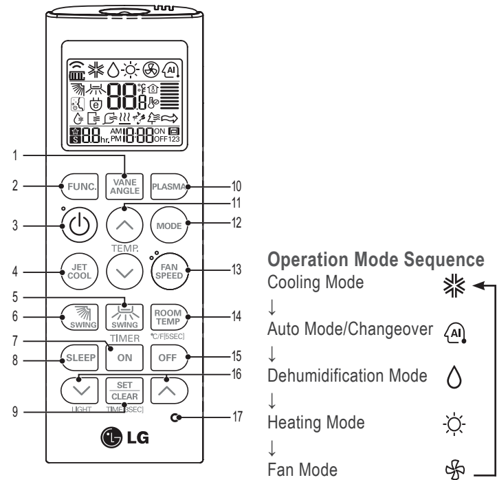
Figure 182:AKB73757604 Wireless Handheld Controller.
