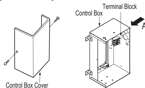
Figure 144: Accessing the Indoor Unit Terminal Block.
