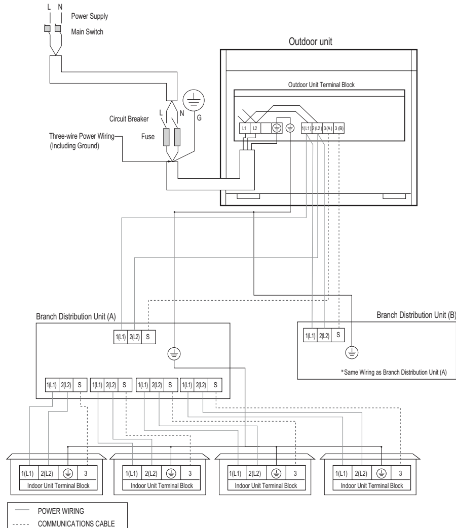
Figure 268: Multi F MAX LMU600HV System Power Wiring and Communications Cable.
