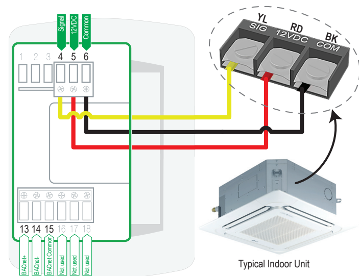
Figure 269: One Example of Indoor Unit to Zone Controller Connection.
