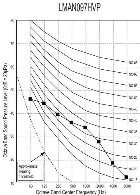
Figure 33: Sound Pressure Level Diagrams.
