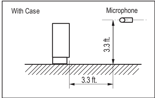
Figure 193: Sound Pressure Level Measurement Location.
