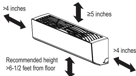
Figure 72: Minimum Clearance Requirements.
