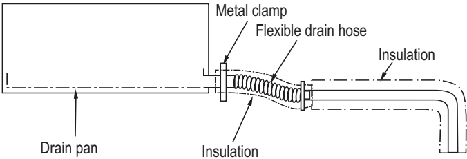
Figure 258:Diagram of an Indoor Unit with a Gravity Drain.
