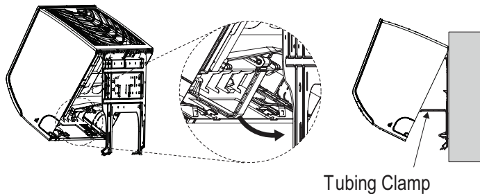
Figure 14: Accessing the Back of the Indoor Unit.
