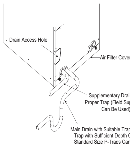
Figure 241: Vertical Primary and Secondary Drain Layout.
