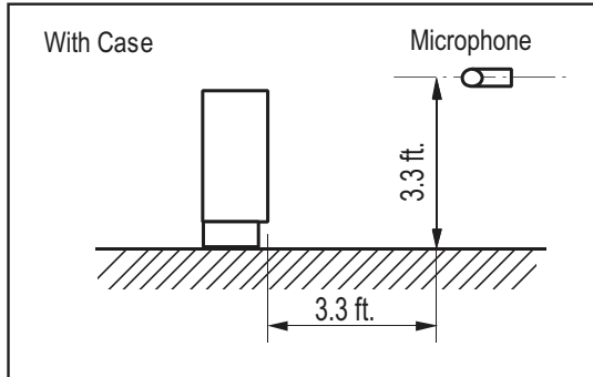
Figure 224: Sound Pressure Level Measurement Location.
