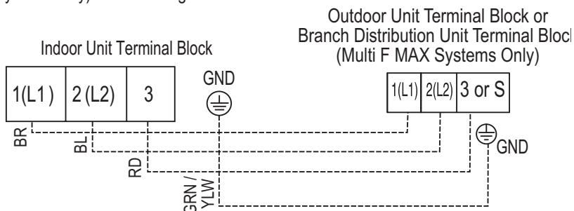
Figure 212: Indoor Unit to Outdoor Unit / Branch Distribution Unit (Multi F MAX systems only) Power Wiring / Communications Cable Connections.
