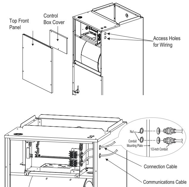
Figure 211: Connecting the Power Wiring and Communications Cable.
