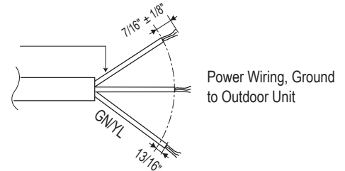
Figure 260: Multi F / Multi F MAX Outdoor Unit Power Wiring.
