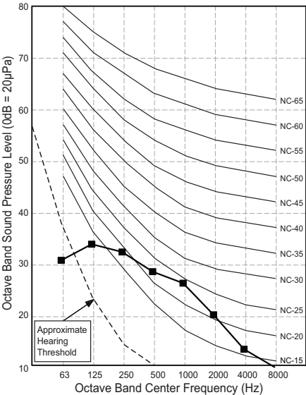
Figure 98: Sound Pressure Level Diagrams. LDN097HV4
