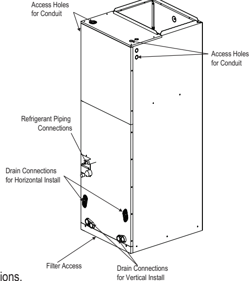
Figure 230:General and Duct Connection Dimensions.
