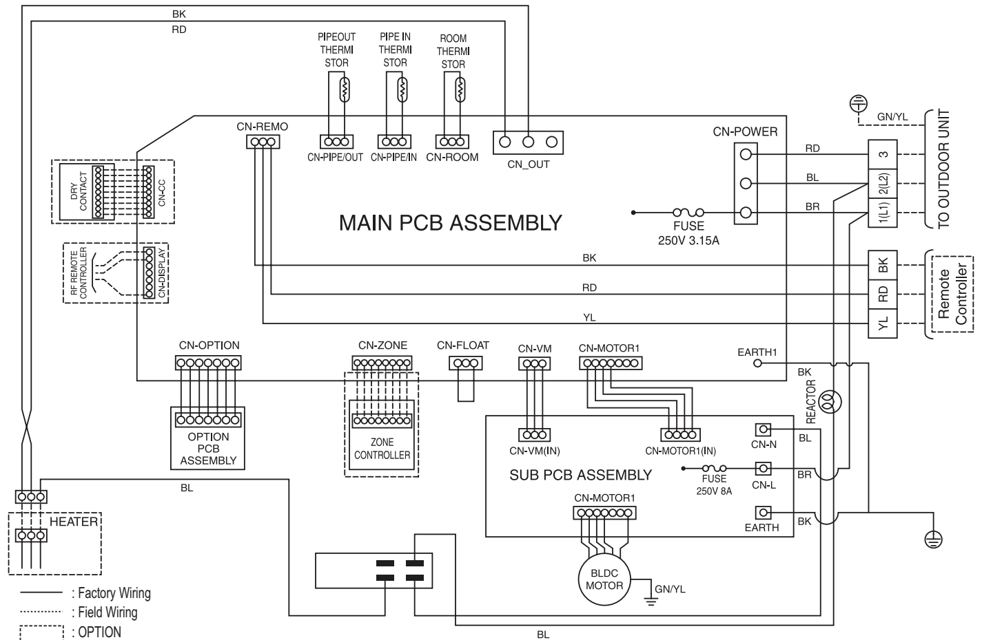
Figure 196: Multi F Vertical-Horizontal Air-Handling Indoor Unit Wiring Diagram.
