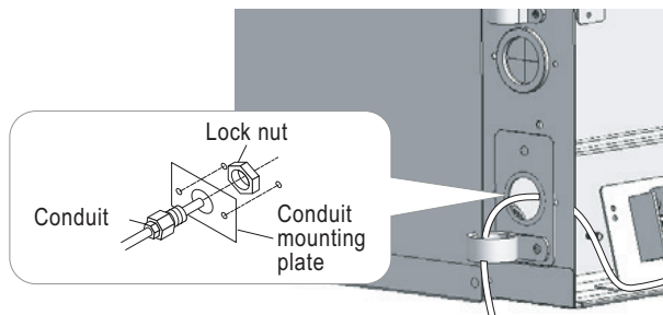
Figure 116: Exterior View of Conduit Installation.
