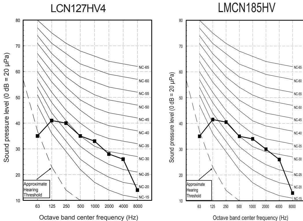
Figure 162: LCN127HV4 and LMCN185HV Sound Pressure Level Diagrams.
