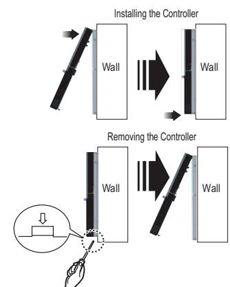
Figure 153: Installing / Removing the Controller.
