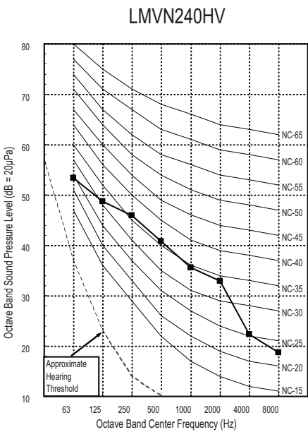
Figure 194: Sound Pressure Level Diagrams.
