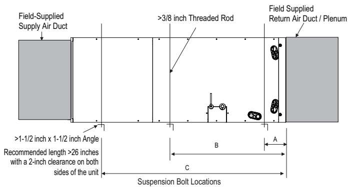
Figure 201:Horizontal Installation.
