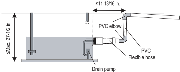
Figure 259:Diagram of an Indoor Unit with a Drain Pump.
