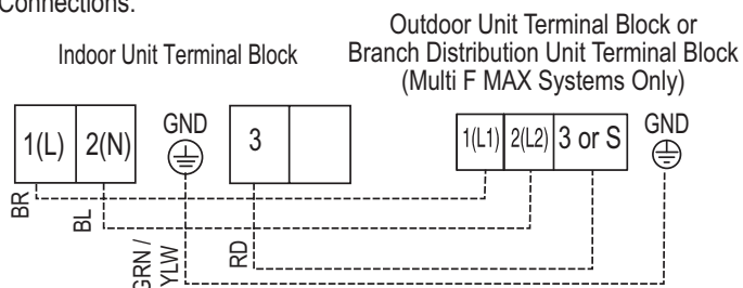
Figure 115: Indoor Unit to Outdoor Unit / Branch Distribution Unit (Multi F MAX systems only) Power Wiring / Communications Cable Connections.
