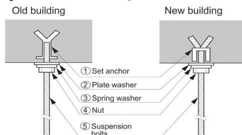
Figure 107: Console Bolt Options.
