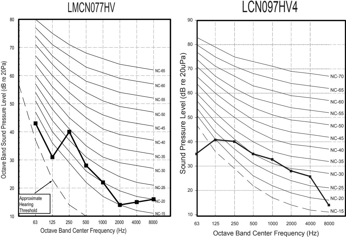
Figure 161: LMCN077HV and LCN097HV4 Sound Pressure Level Diagrams.
