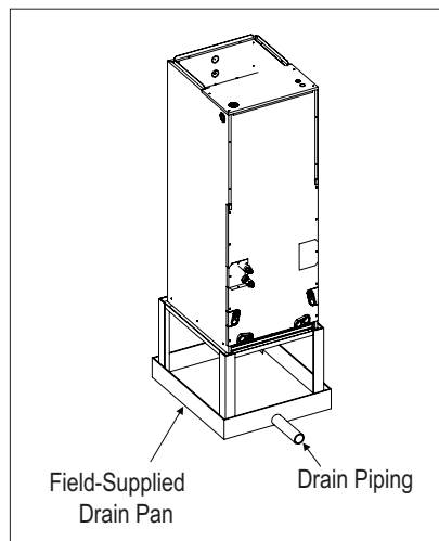
Figure 237: Typical Vertical Up/Down Installation Drain System.
