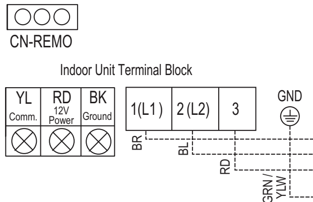
Figure 214:Wired Controller Connection on the Indoor Unit Terminal Block.
