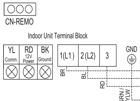
Figure 149: Wired Controller Connections on the Indoor Unit Terminal Block.
