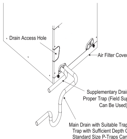
Figure 207: Vertical Primary and Secondary Drain Layout.
