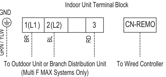
Figure 88:Wired Controller Connection on Indoor Unit Terminal Block—LSN180HSV5 and LMN249HVT Models.
