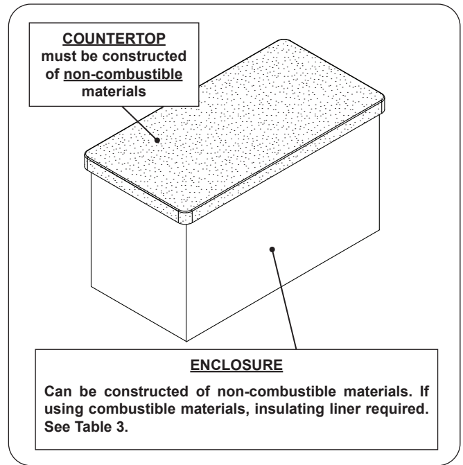
Fig. 9-1 Enclosure detail
