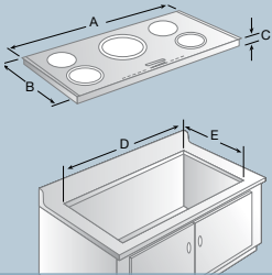
36" Induction Cooktop
