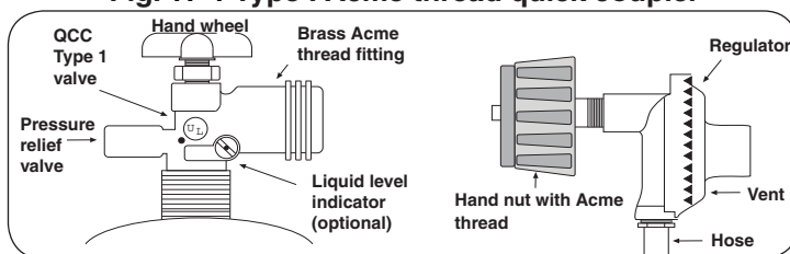
Fig. 17-1 Type I Acme thread quick coupler
