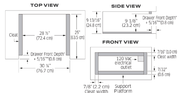
FLUSH INSTALLATION CUTOUT DIMENSIONS
