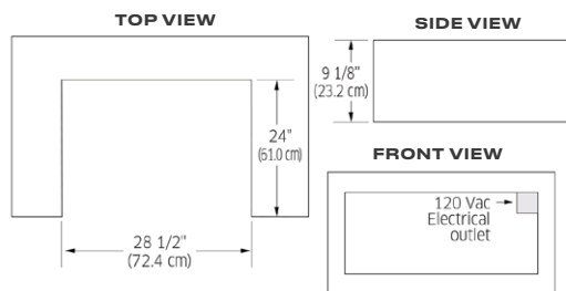
STANDARD INSTALLATION CUTOUT DIMENSIONS
