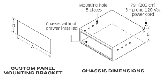
CHASSIS DIMENSIONS
