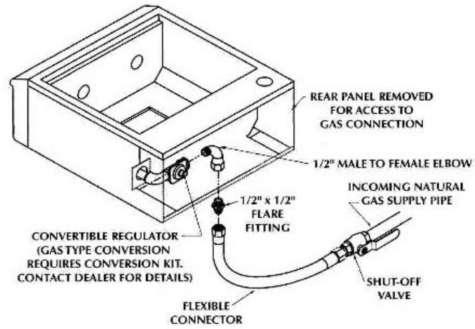
Figure 3- Natural Gas Connection
