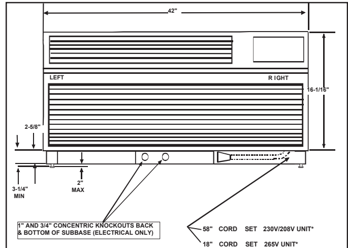
58" LCDI CORD SET — 230V/208V UNIT*
