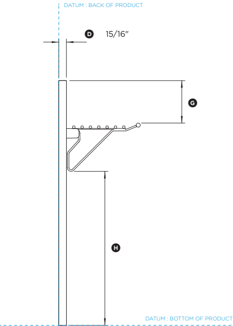
PROFILE VIEW
