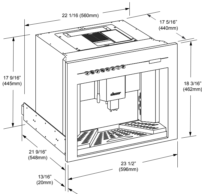
OVERALL DIMENSIONS
