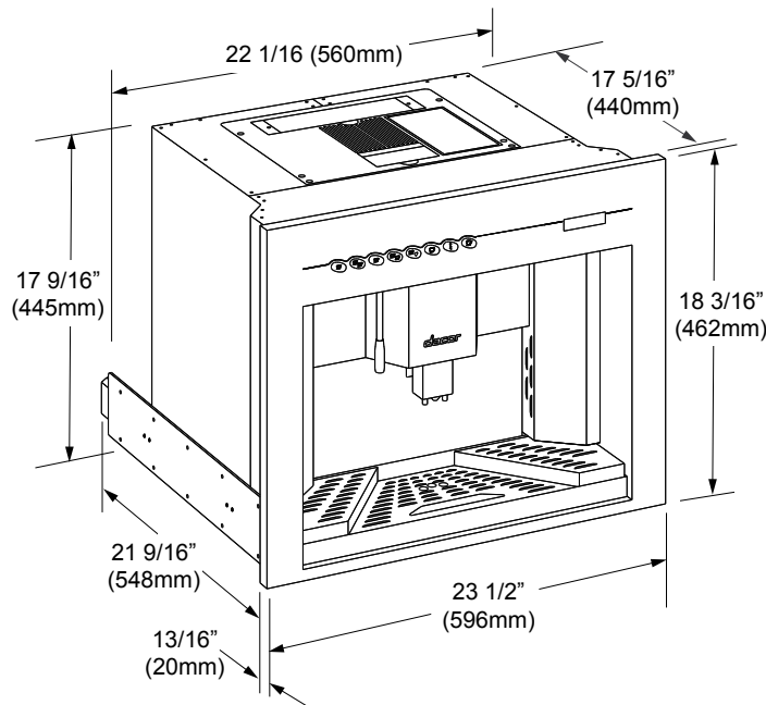
OVERALL DIMENSIONS
