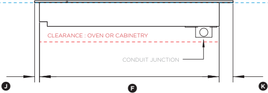
PROFILE VIEW
