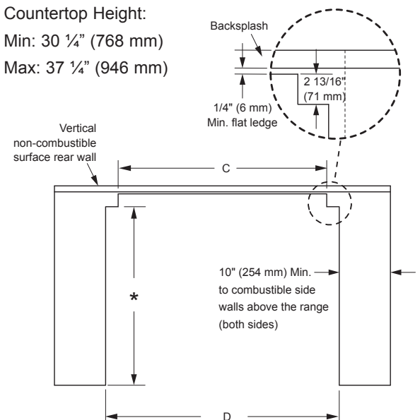
CABINET CUTOUT TOP VIEW
