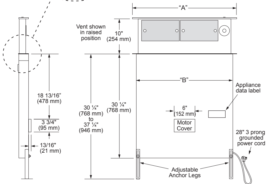
ERVXX-ER OVERALL DIMENSIONS SIDE VIEW
