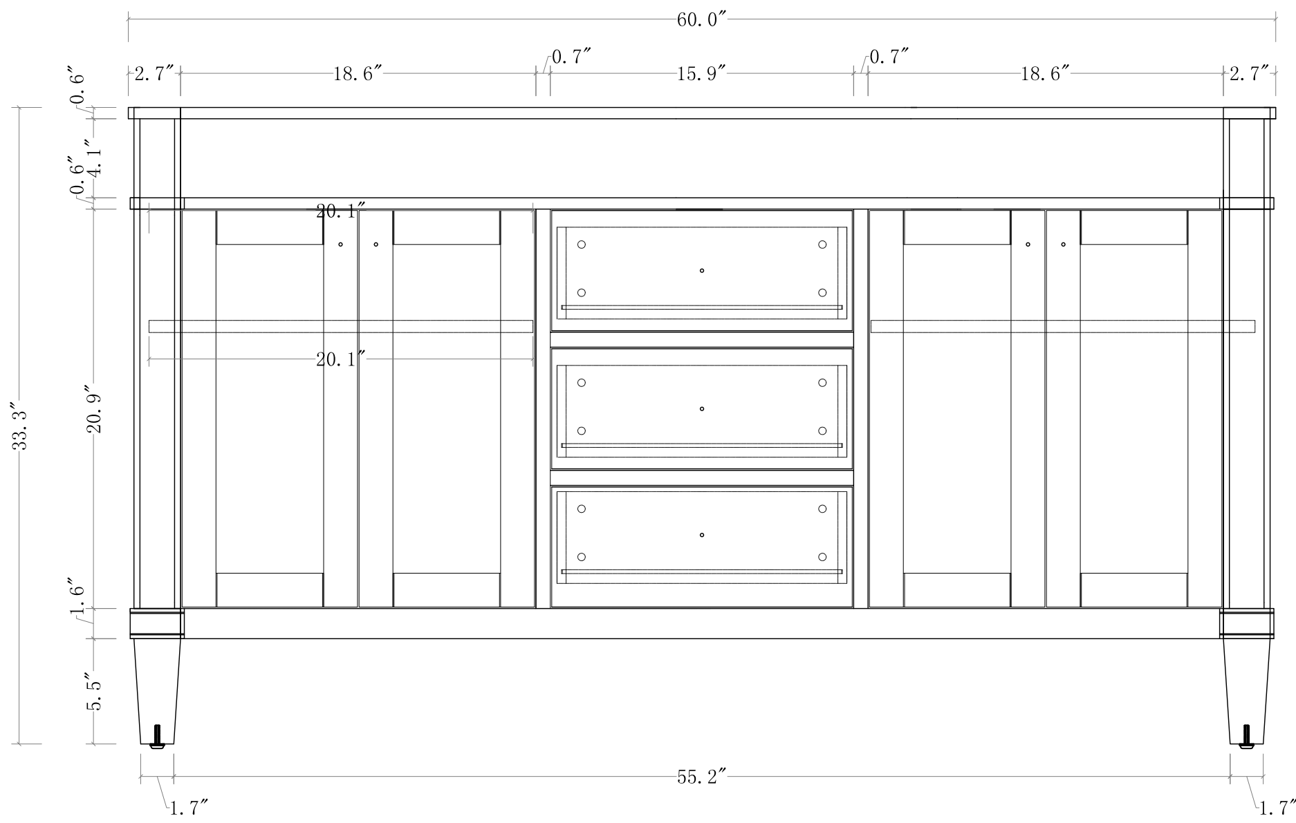
FRONT VIEW
