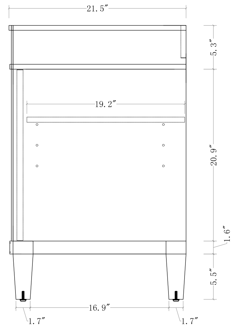
SIDE VIEW
