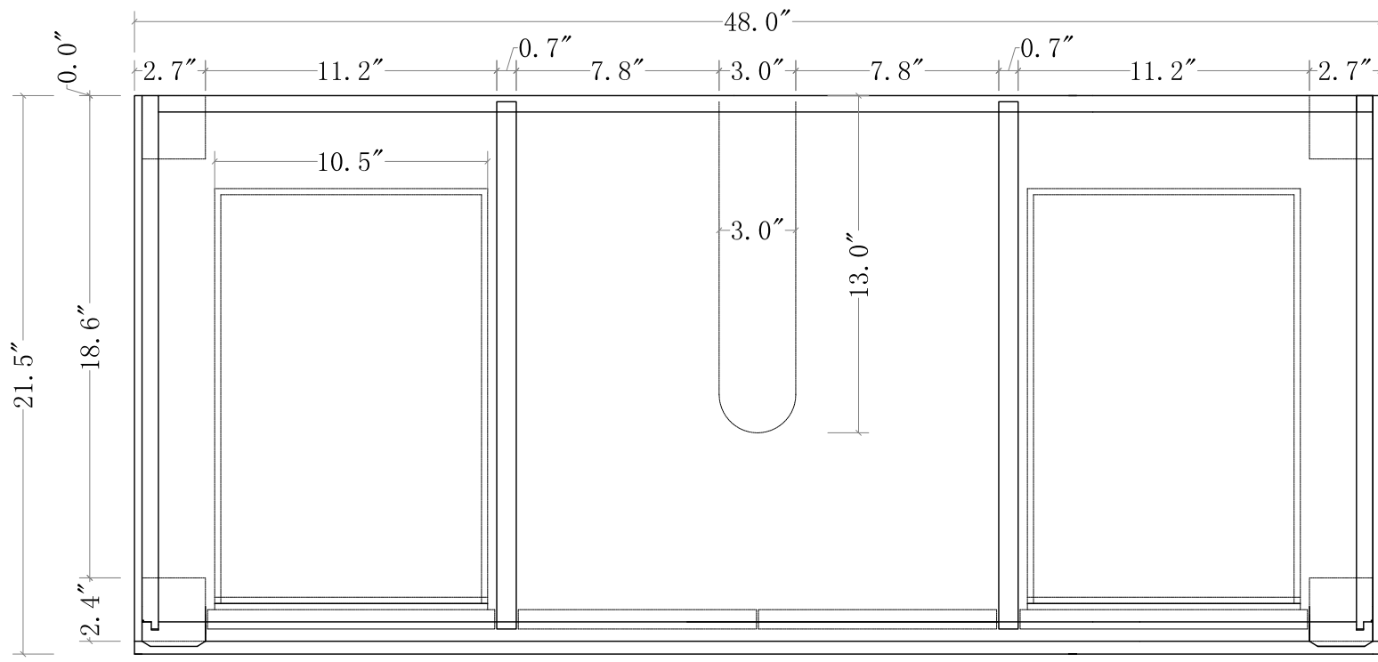
TOP VIEW
