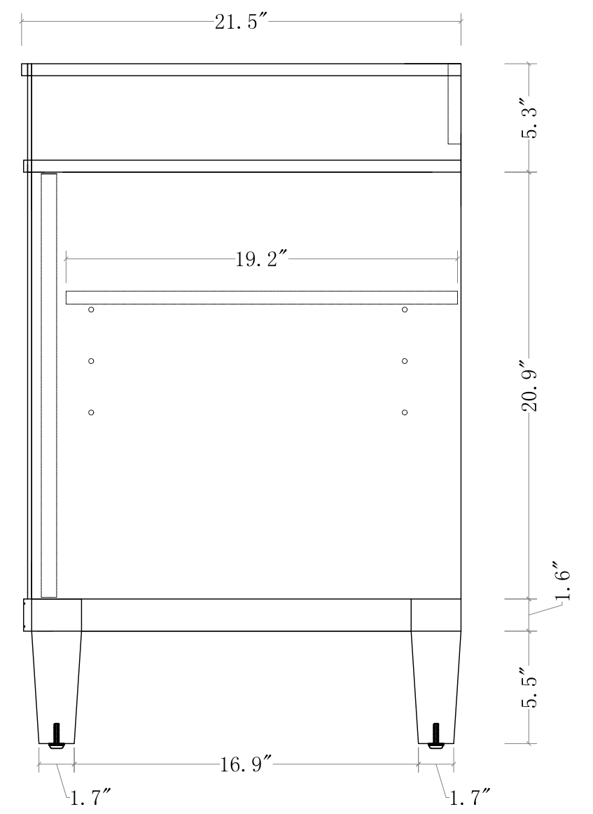
SIDE VIEW
