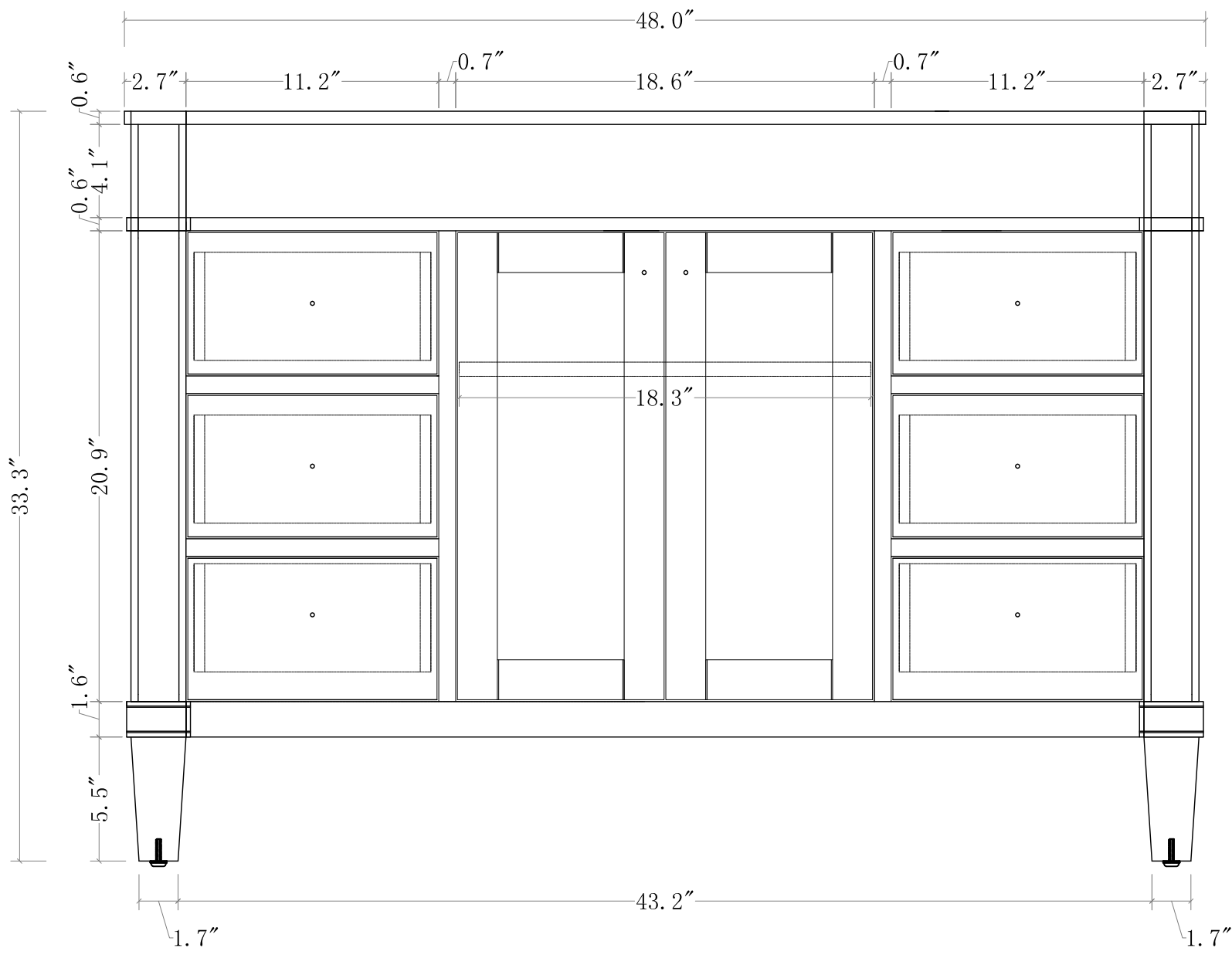
FRONT VIEW
