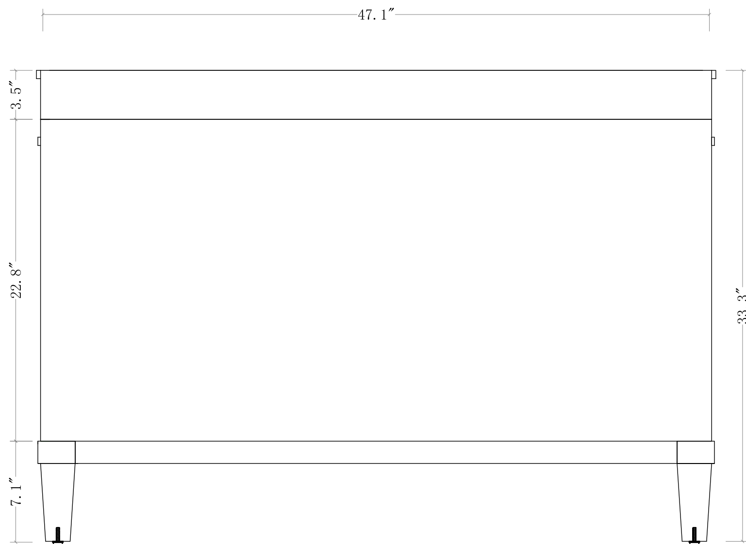
BACK VIEW
