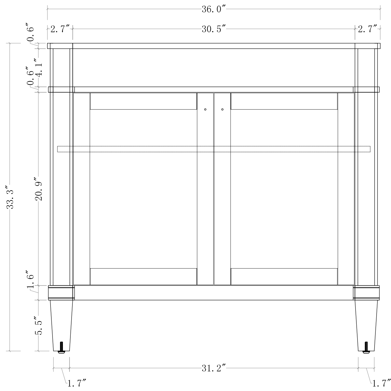
FRONT VIEW
