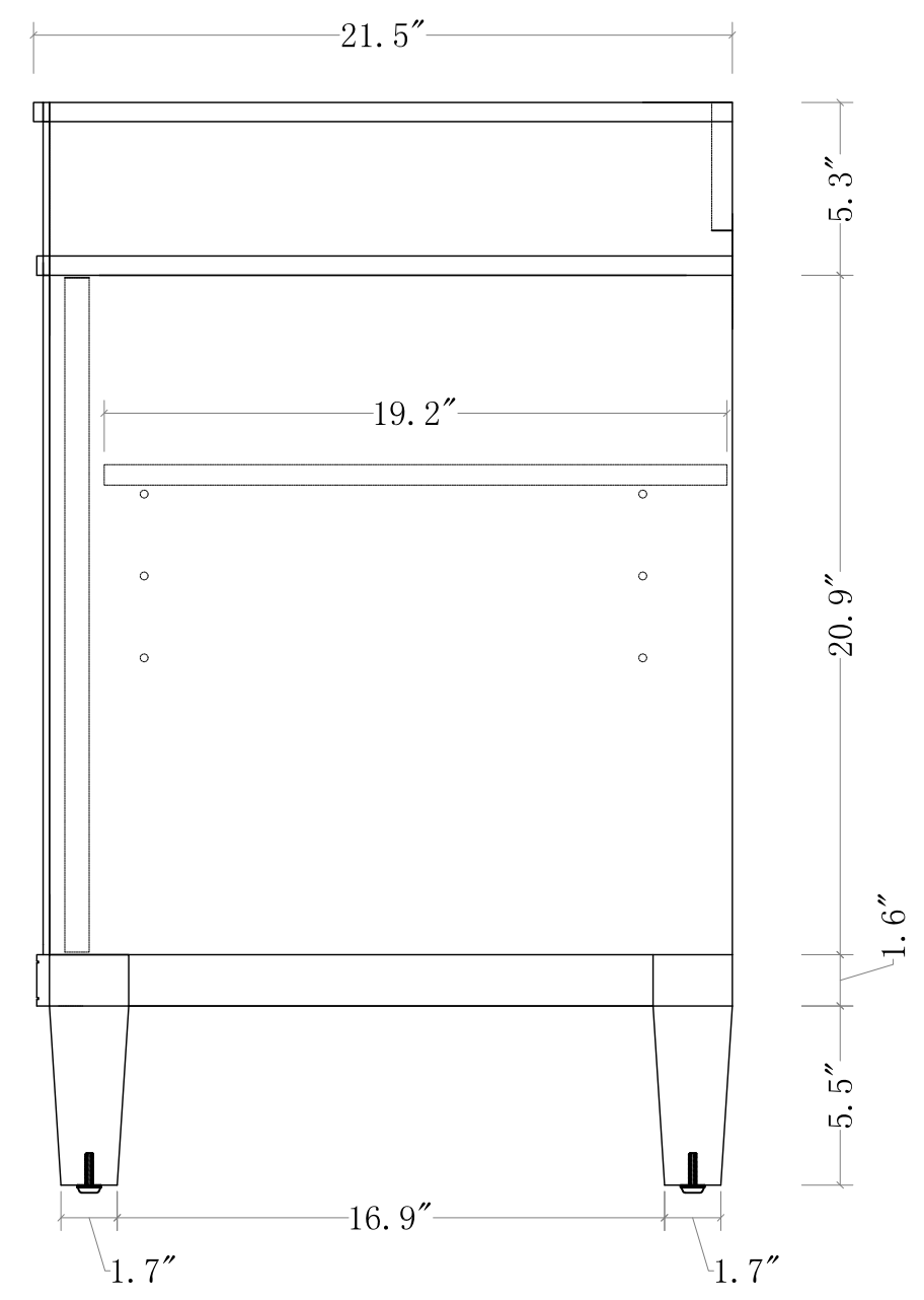
SIDE VIEW
