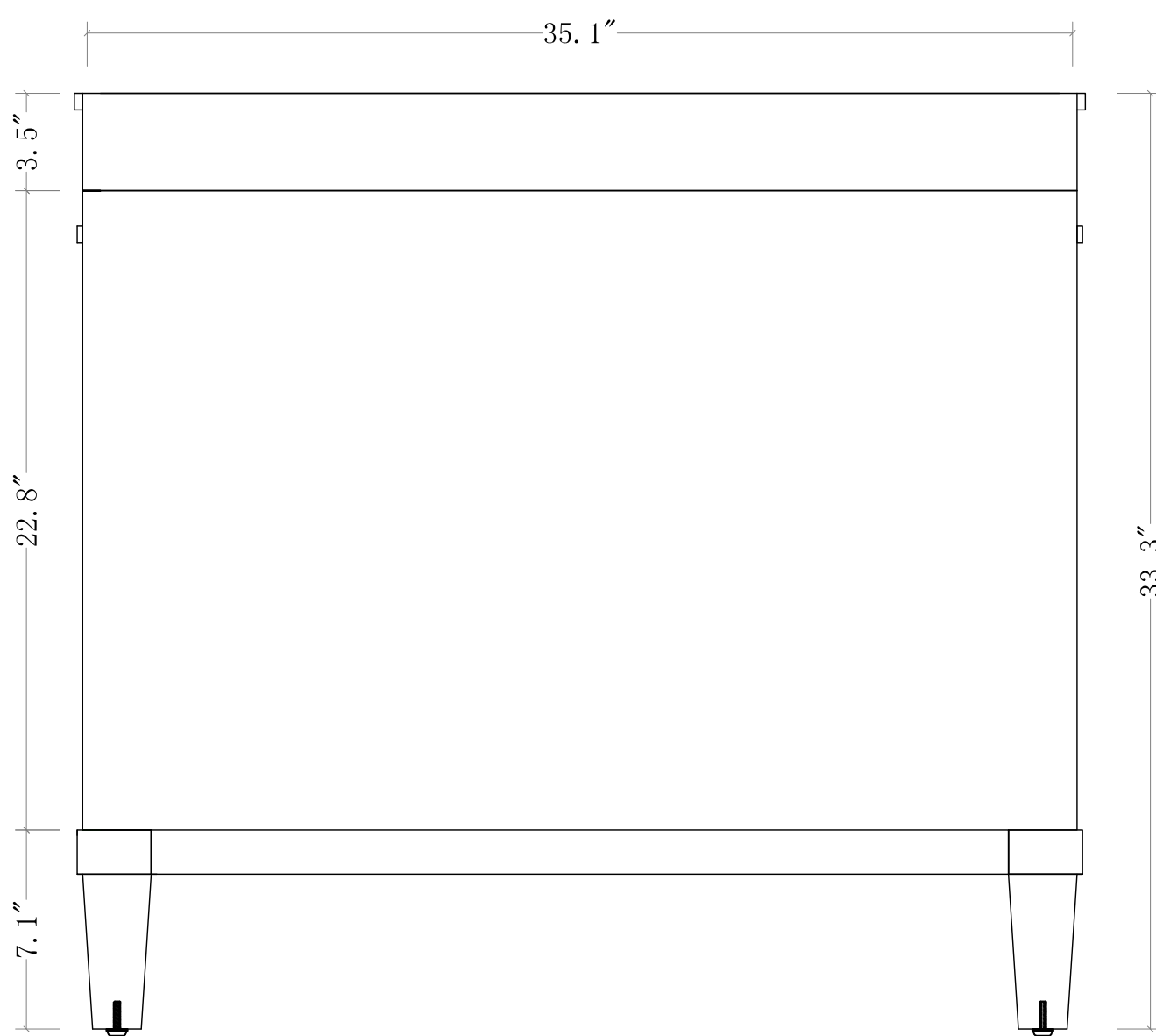
BACK VIEW
