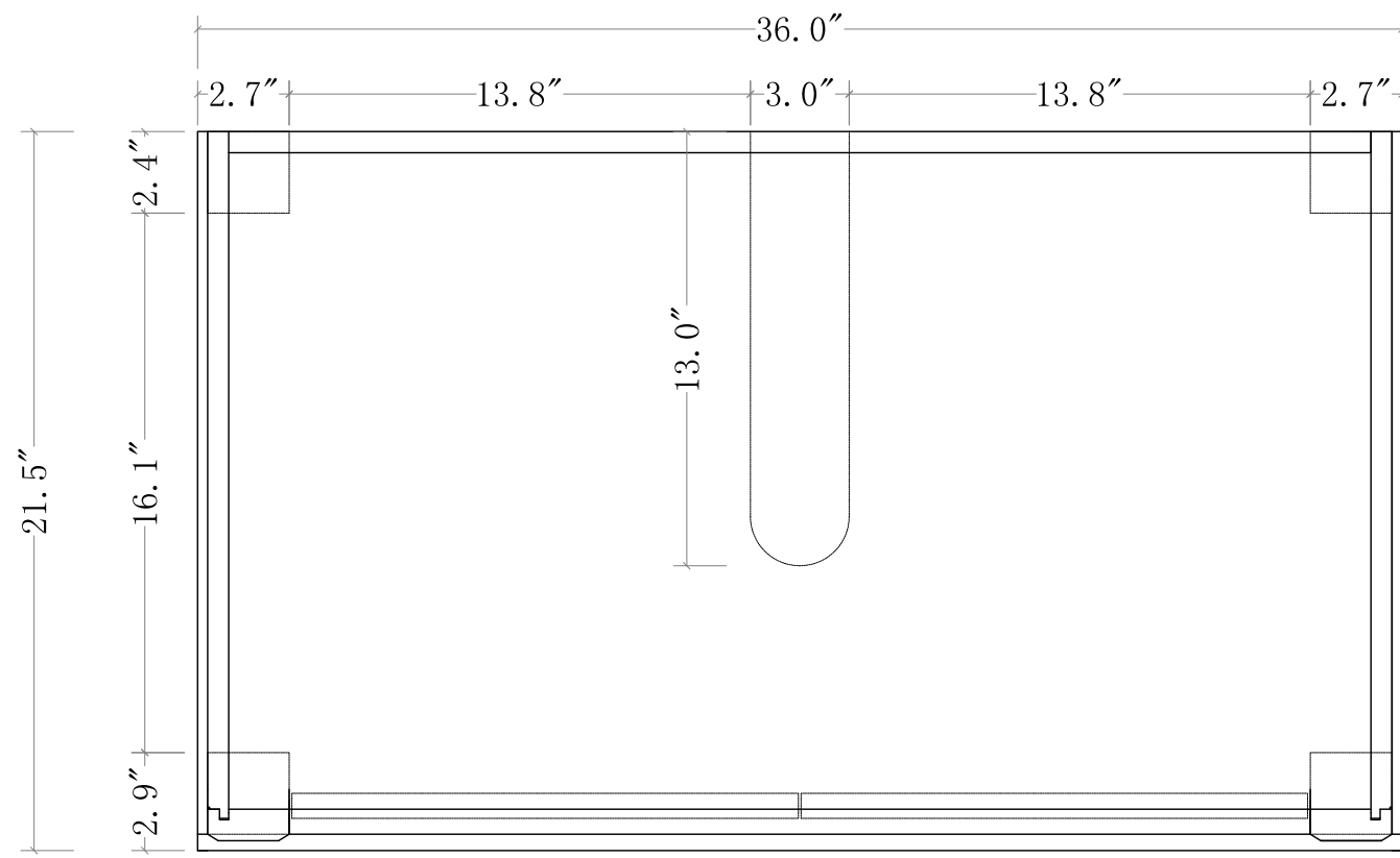
TOP VIEW
