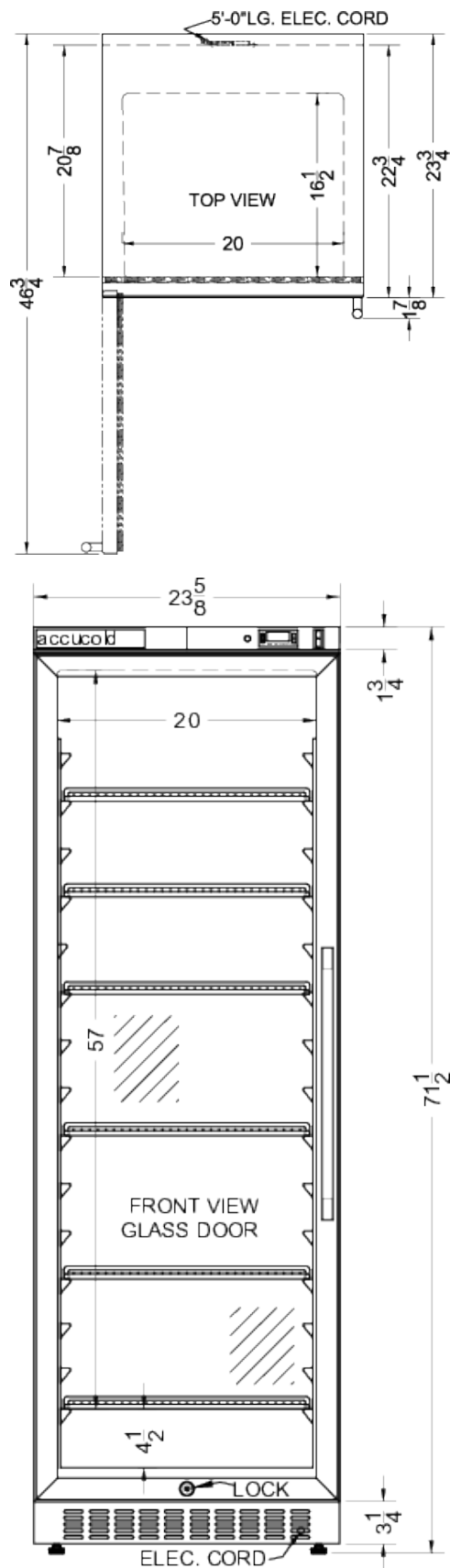
Puretherm Warming Cabinet
