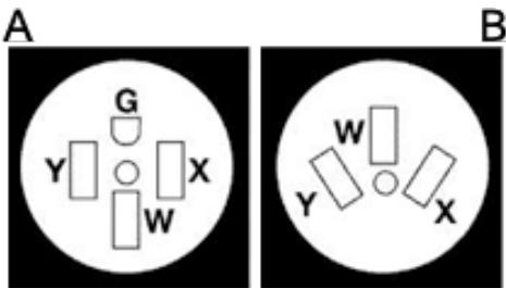
A 4-wire wall receptacle. B 3-wire wall receptacle (10-50R)
