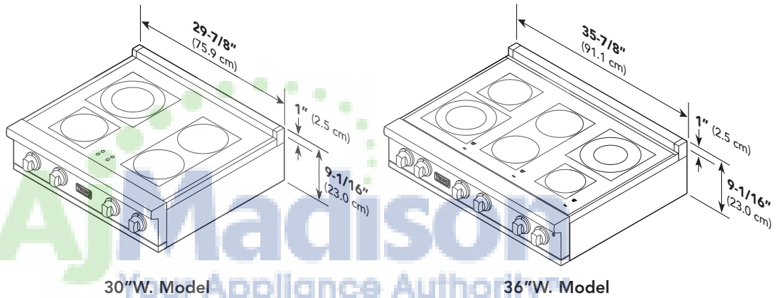
VERT530-4B Professional 30"W. Four-Burner Rangetop
