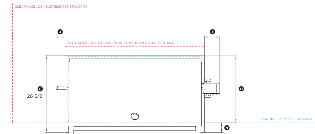
PLAN VIEW
