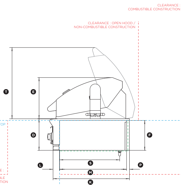
PROFILE VIEW
