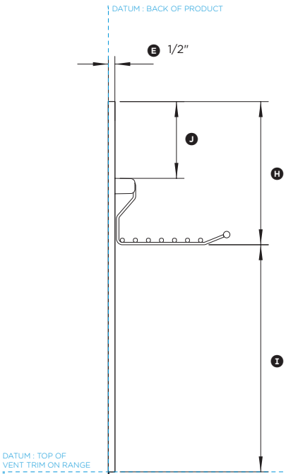
PROFILE VIEW
