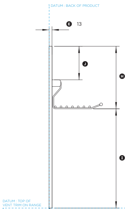
PROFILE VIEW
