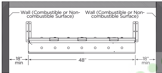
INSTALLATION TO COMBUSTIBLE AND NON-COMBUSTIBLE CONSTRUCTION (FRONT VIEW)
