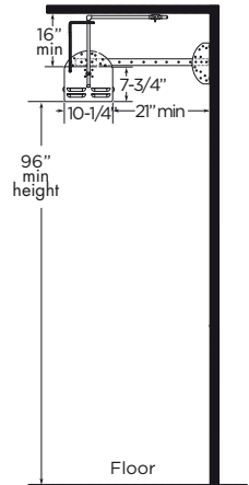
0° INSTALLATION TO COMBUSTIBLE (SIDE VIEW)
