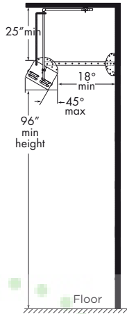
45° INSTALLATION TO COMBUSTIBLE (SIDE VIEW)
