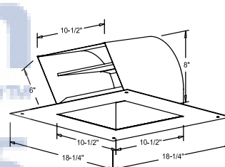
RC - 10 ROOF CAP - 10"
