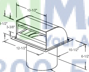
WC - 8 WALL CAP - 8"
