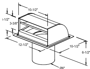
WC - 6 WALL CAP - 6"
