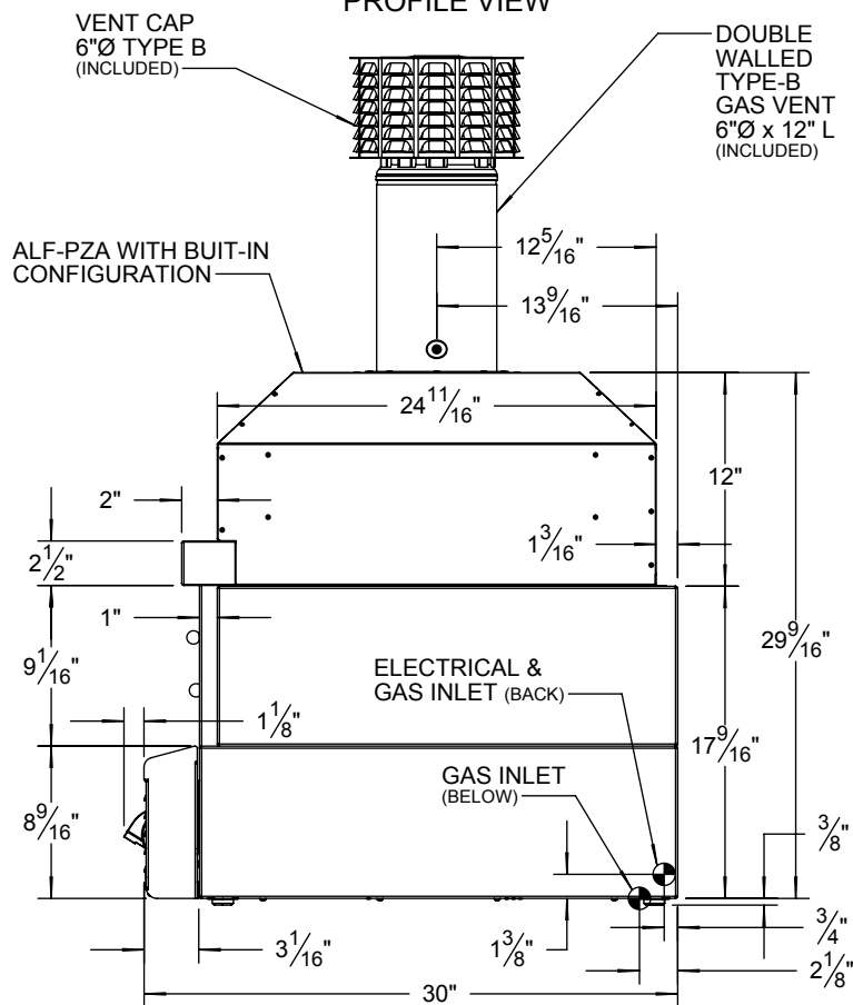
PROFILE VIEW
