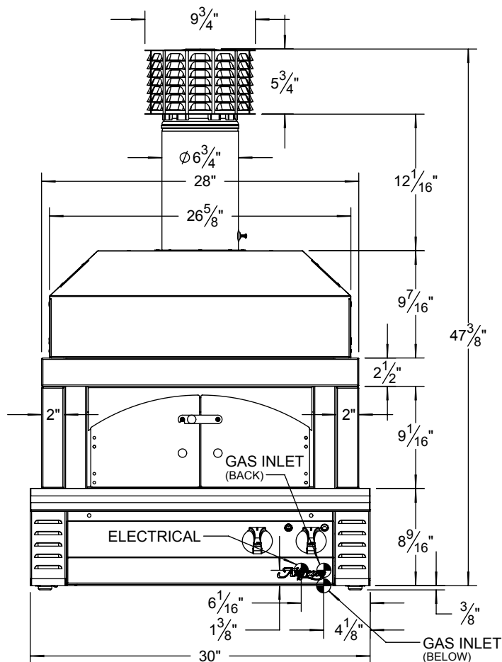
FRONT VIEW
