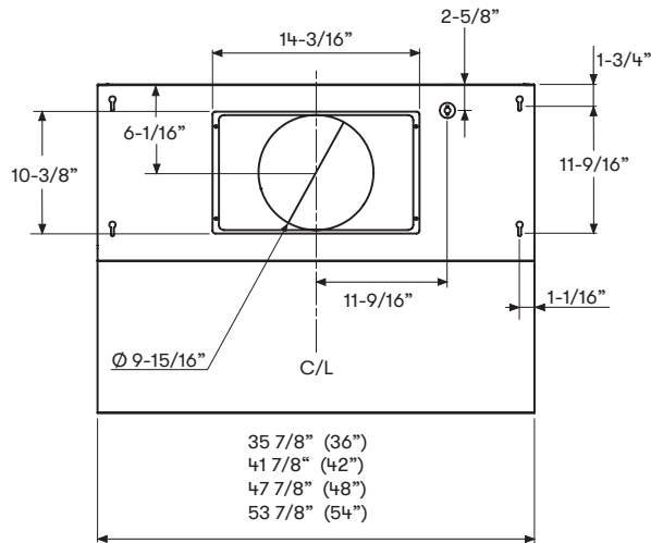
Back View Ducting & Electrical Dimensions
