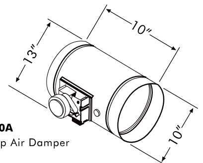
MUA008A Make-Up Air Damper
