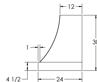
48" SIDE VIEW
