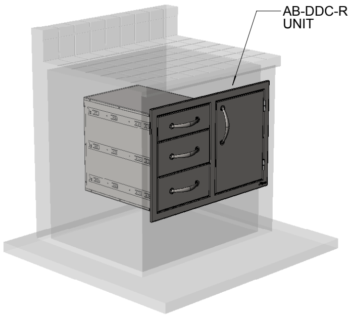
TYPICAL AB-DDC INSTALLATION
