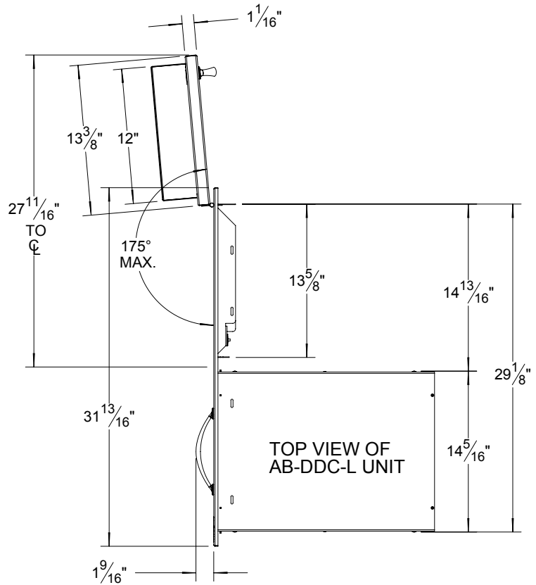
FOR AB-DDC-R UNIT REVERSE DIMENSIONS
