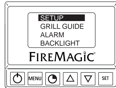
Fig. 19-2 Menu screen
