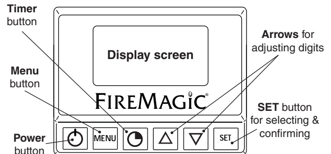
Fig. 18-2 Orientation
