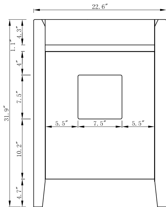
BACK VIEW
