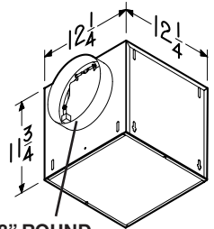
8" ROUND DUCT CONNECTOR
