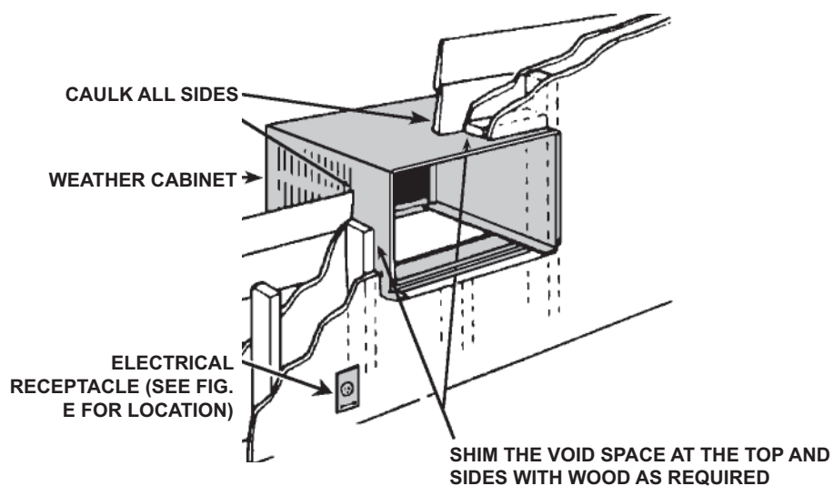
FIGURE C FRAME WALL CONSTRUCTION
