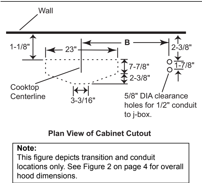
Figure 12: Transition and Conduit Locations
