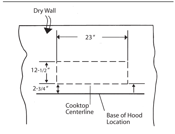
Figure 6: Cutout Dimensions
