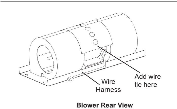
Figure 14: Blower Rear View
