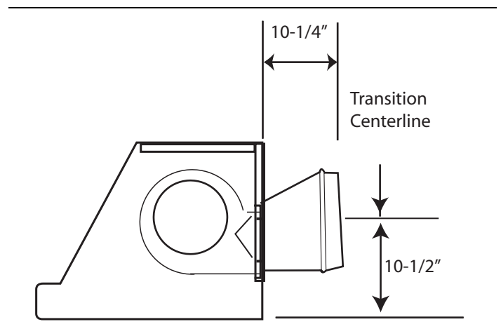
Figure 7: Transition Centerline for Horizontal Discharge
