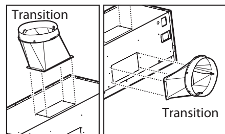
Vertical discharge
