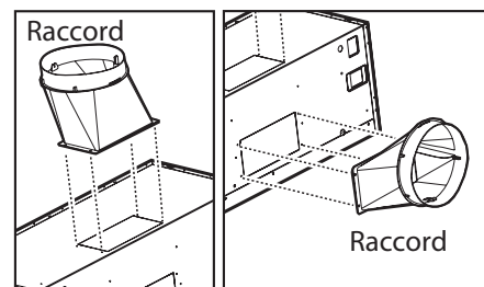
Evacuation verticale
