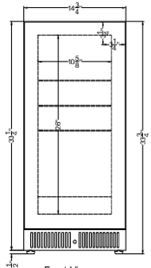
Front View
