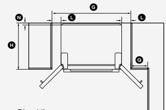
Plan View Flush with refrigerator door - 90° door rotation
