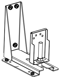
Support antibasculement (1)
