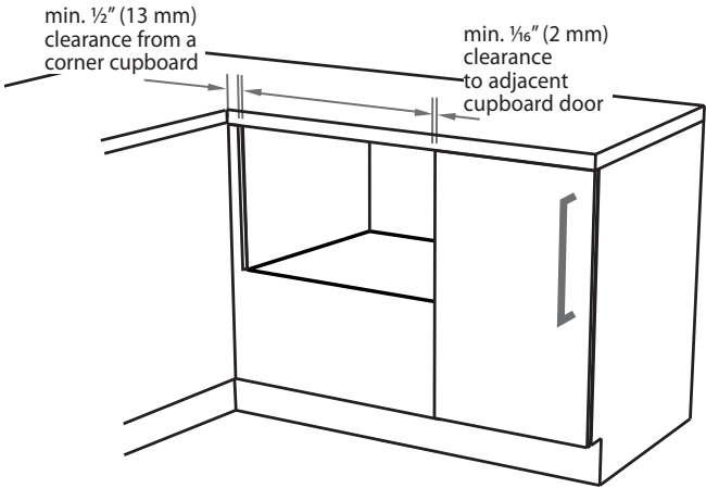
Minimum clearances from adjacent cabinetry
