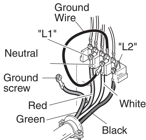
4-wire Cord Installed
