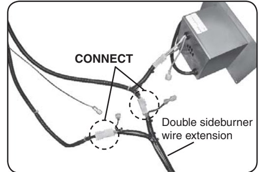
Fig. 13-2 Sideburner extension connections
