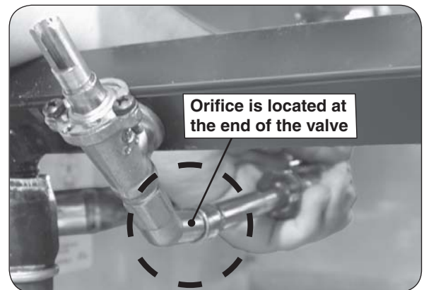
Fig. 17-2 Orifice location
