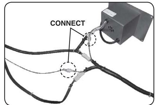
Fig. 13-3 Connect ground wires
