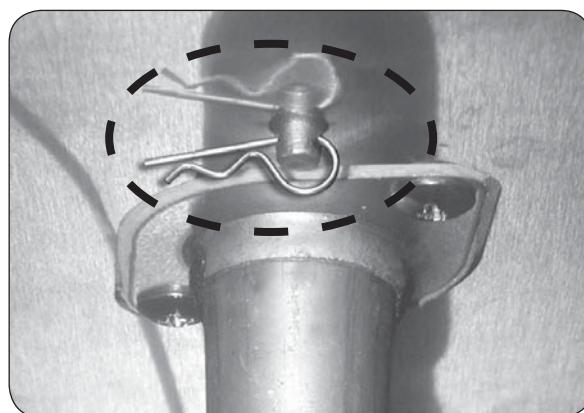
Fig. 16-2 Remove burner clip
