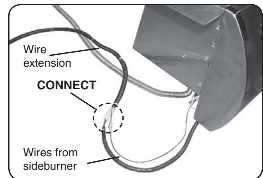
Fig. 13-4 Connect extension to sideburner
