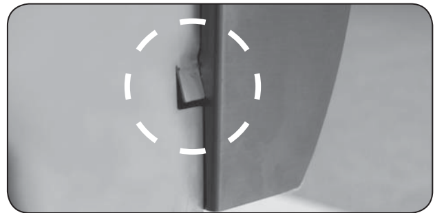
Fig. 14-3 Tab slightly bent in for clearance
