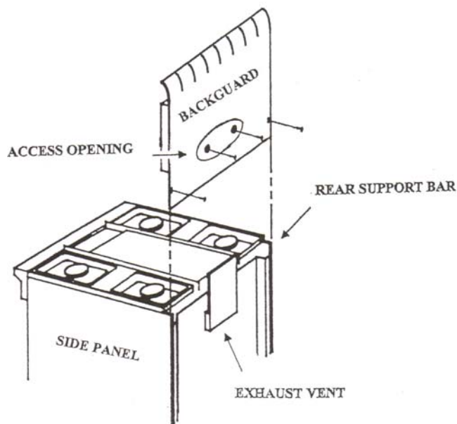
BACKGUARD INSTALLATION
