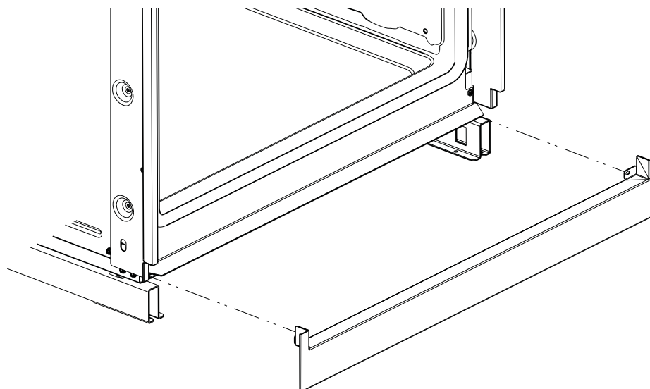
DWO's with pedestals
