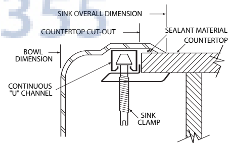
Installation Detail
