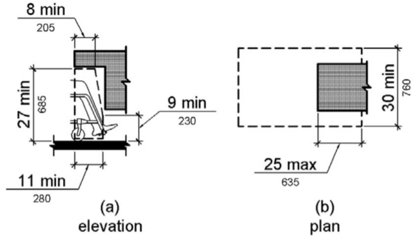
Figure 306.3 Knee Clearance
