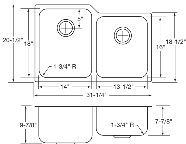
Model PLAUH3120R Illustrated
