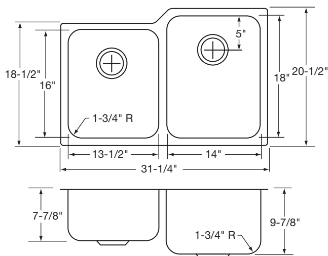
Model PLAUH3120L Illustrated
